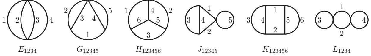
FIG. 3.1: The Feynman diagram topologies contributing to the 3-loop effective potential, with numerals indicating the ordering of subscripts denoting propagator types ( S , F , \overline{F} , V , or g ) as well as the ordering of the corresponding squared mass arguments.
