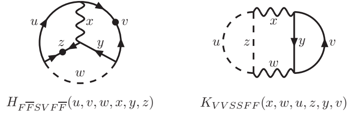
FIG. 3.2: Examples of the Feynman diagram labeling scheme used in this paper, for the diagrams with loop integral functions denoted H_{F\overline{F}SVF\overline{F}}(u, v, w, x, y, z) and K_{VVSSFF}(x, w, u, z, y, v) . Solid lines with arrows represent helicity-preserving fermion propagators. Solid lines with a dot and clashing arrows represent a helicity-violating fermion propagator. Dashed lines indicate a real scalar propagator, and wavy lines stand for real vector propagators. The squared masses are denoted by u, v, w, x, y, z as labeled.
