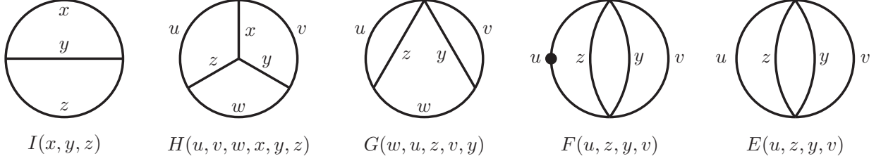
FIG. 2.1: The topologies for the 2-loop and 3-loop basis vacuum integral functions used in this paper. The large dot in F(u, z, y, v) corresponds to a derivative with respect to the u squared mass argument. The function \overline{F}(u, z, y, v) is the same as F(u, z, y, v) but with a subtraction to render it infrared finite in the limit u \rightarrow 0 . In each case, counterterms have been included to make the integrals finite as the ultraviolet regulator \epsilon \rightarrow 0 . See ref. [51] for the precise definitions and more information.
