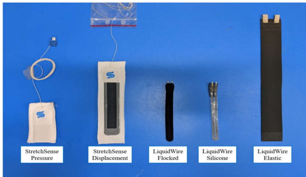
Figure 1. Different wearable stretch sensors used by the current research team. From left to right: (1) StretchSense Pressure Sensor, (2) StretchSense Displacement Sensor, (3) LiquidWire Flocked Sensor, (4) LiquidWire Silicone Sensor, and (5) LiquidWire Elastic Sensor.
