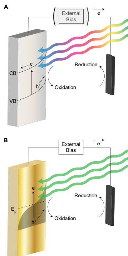
Figure 1. Comparison of the Mechanism of Photoexcitation of Charge Carriers in PEC and PEEC
