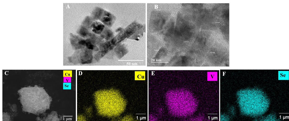
Fig 2. (A) Low-resolution TEM images. (B) HRTEM images. (C) SEM image of synthesized CVSe NCs. (D–F) SEM-EDS elemental mapping of CVSe NCs.
