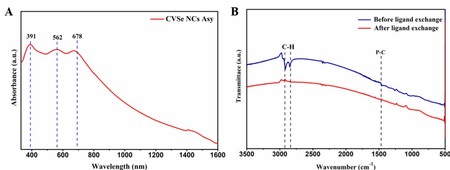
Fig 4. (A) UV-Vis-NIR spectra of the synthesized CVSe NCs in ethanol (B) FTIR spectra of the as-synthesized CVSe NCs (blue line) and CVSe with ligand exchange (red line).
