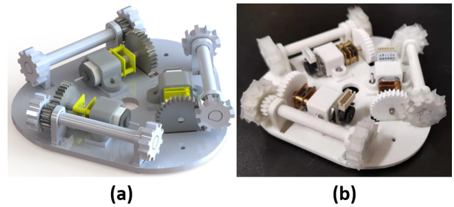
Fig. 4. (a) CAD rendering of gear transmission design, (b) Fabricated gear transmission design.
