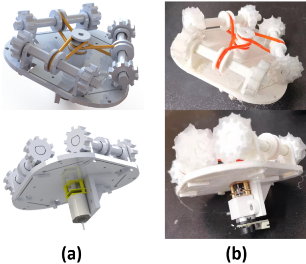
Fig. 5. (a) CAD rendering of belt transmission design, (b) Fabricated belt transmission design.
