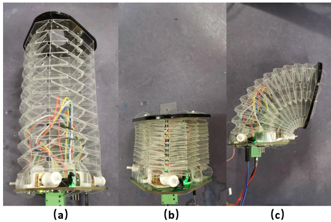
Fig. 3. (a) Fully stretched origami module, with the length of 148mm, (b) Fully compressed origami module, the length is 57mm, 38% of the maximum length, (c) Maximum bending angle of our origami module is 106 deg.
