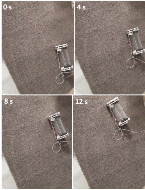
Fig. 9. Salamanderbot climbing on a 60 deg carpet surface slope.
