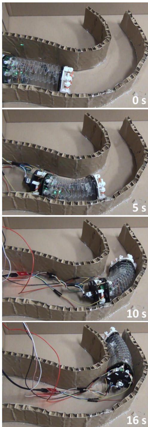
Fig. 6. Salamanderbot going through a maze.
