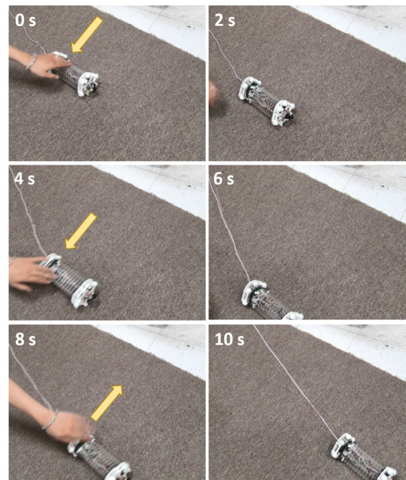
Fig. 8. During the experiment, Salamanderbot was turned over several times, while the velocity stayed the same. The yellow arrows show the turning over directions.
