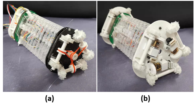
Fig. 1. (a) Salamanderbot with belt transmission design, (b) Salamanderbot with gear transmission design.
