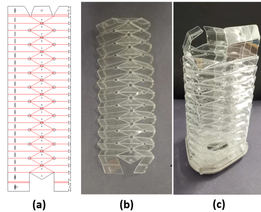
Fig. 2. (a) Yoshimura origami pattern, (b) Folded Yoshimura origami pattern with PET sheet, (c) Combine three pieces of (b) to get a triangular origami module.
