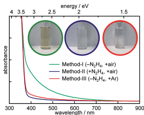
Fig. 2 Electronic absorption spectra of colloidal SrTiO 3 NCs dispersed in hexanes prepared by method-I (green), method-II (blue) and method-III (red). Optical densities were matched at ~350 nm. Color photographs of NCs dispersed in hexanes are shown in insets.
