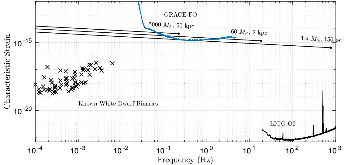
FIG. 4. Estimates of the characteristic strain sensitivity of GRACE-FO along with the expected strain from known white dwarf binaries [22–25] and a sensitivity curve for LIGO's second observing run [26]. Also shown are lines that correspond to the predicted characteristic strain of an equal component-mass 1.4 M_\odot binary at 150 pc, a 60 M_\odot at 2 kpc, and a 5000 M_\odot at 50 kpc [21]. The points at the end of each line note the merger frequency for the corresponding system. These approximations are only valid for the inspiral phase of binary evolution.
