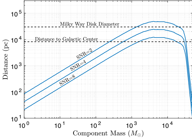
FIG. 5. Maximum detectable distance for equal component-mass binaries with SNR thresholds of 2, 4, and 8. For systems with component-mass of 2000–10000 M_\odot the detection volume encompasses most of the Milky Way.
