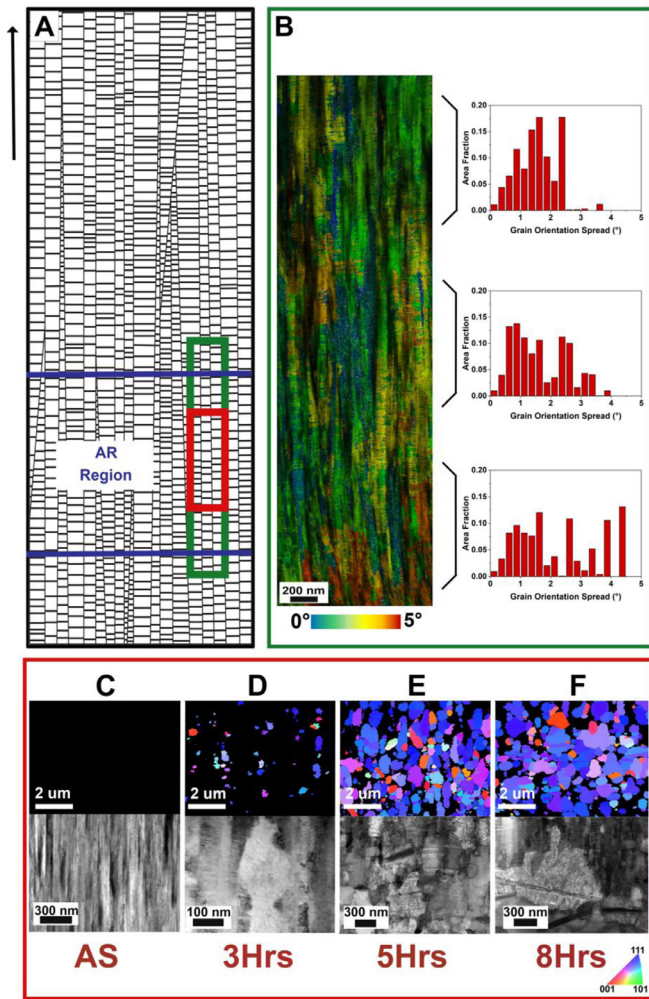
Fig. 2. (A) Schematic of a representative cross-section of the as-sputtered film highlighting the region expected to undergo abnormal recrystallization delineated by blue lines. Growth direction is shown by arrow to the left. This region includes a green rectangle representing (B) and a red rectangle representing (C-F). Where (B) shows the GOS map and corresponding distribution plots, which reveals a gradient in GOS. (C-F) highlight the EBSD scans (top) and BF-STEM images (bottom) representing the microstructural evolution of the abnormal recrystallization region in (C) the as-sputtered condition and after aging treatments of (D) 3 h, (E) 5 h, and (F) 8 h. IPF triangle is shown to the bottom right of the scans. (For interpretation of the references to color in this figure legend, the reader is referred to the web version of this article.)
