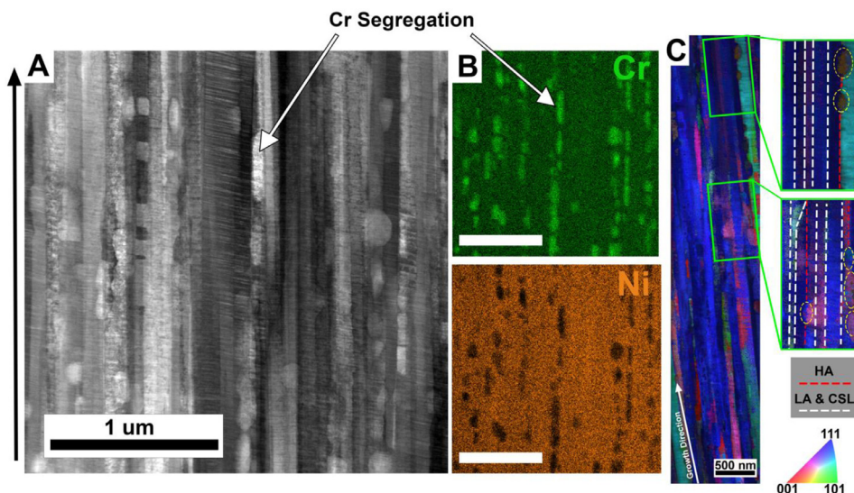
Fig. 3. (A) BF-STEM image of the 3-hour aged sample of the upper portion of the film and (B) corresponding EDS maps highlighting Cr segregation where white scale bars are 1 \mu\text{m} . (C) ACOM scans of representative region, where green insets highlight select GBs with red dotted lines indicating HAGBs and white dotted lines indicating low angle (LA) GBs and coincident site lattice (CSL) GBs. Cr precipitates are encircled with yellow dotted lines. IPF triangle is shown to the right of the scan. (For interpretation of the references to color in this figure legend, the reader is referred to the web version of this article.)
