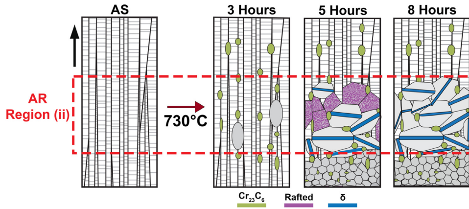
Fig. 8. Schematic overview of the microstructural evolution of the sputtered Inconel 725 film at different aging times that presents the changes in grain morphology, precipitate formation, and development of a heterogeneous microstructure. The arrow to the left indicates the growth direction of the film and the red dotted box highlights the AR region.
