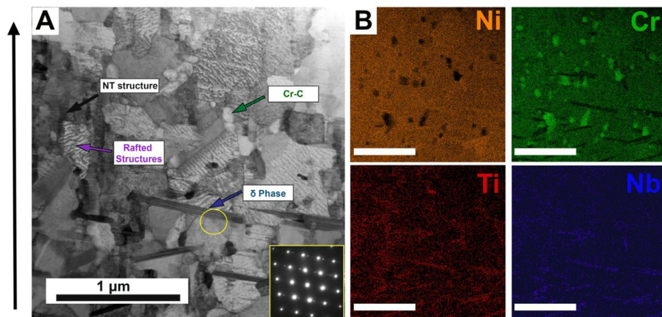
Fig. 6. (A) BF-STEM image of the 5-hour aged sample illustrating the heterogeneous precipitate and microstructural behavior in the AR region with inset SAED pattern confirming the presence of \delta precipitates. (B) EDS maps of Ni, Cr, Ti, and Nb highlighting location of different precipitates where white scale bars are 1 \mu\text{m} .
