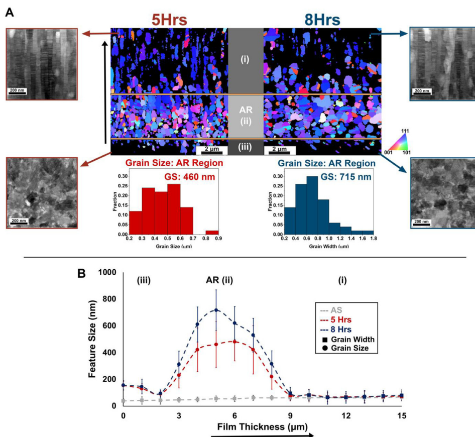
Fig. 4. (A) EBSD maps of cross-section of heterogenous structured achieved at aging times of 5 and 8-hours (top) with respective grain size distributions of grains in the AR region (ii) (bottom). Insets highlights characteristic microstructures of the region (i) and region (iii) at the different aging times. IPF triangle is shown to the right of the scans. (B) Feature size is plotted as a function of film thickness for films in the as-sputtered (AS) condition (grey), and after aging at 5 (red) and 8 h (blue), where filled squares indicate columnar grain width measurements and filled circles indicate equiaxed grain size measurements. The arrows indicate the growth direction of the film. (For interpretation of the references to color in this figure legend, the reader is referred to the web version of this article.)
