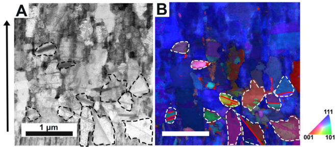
Fig. 5. (A) BF-STEM images and (B) corresponding ACOM scans of the AR region in the 5-hour aged sample, highlighting ALGs governed by different thermal processes. Randomly oriented recrystallized grains are highlighted by dashed black and white lines. White scale bar is 1 \mu\text{m} and IPF triangle is shown to the right of the scan.
