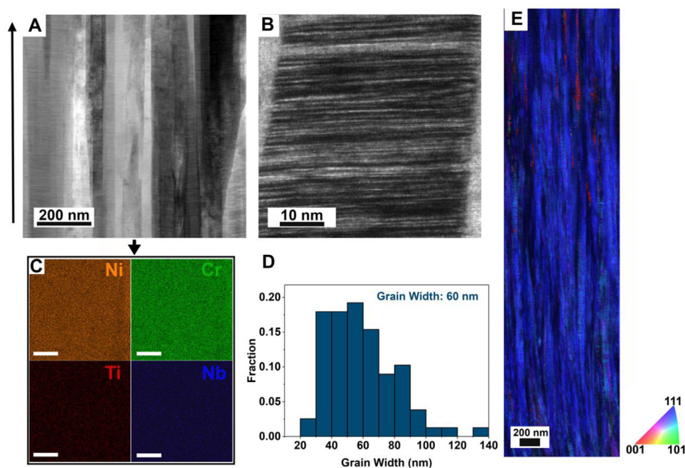
Fig. 1. (A) BF-STEM image showing the nanoscale columnar structure of the as-sputtered Inconel 725 sample, with (B) bright field TEM images highlighting density of nanotwins. (C) EDS maps of corresponding STEM image in (A) of Ni, Cr, Ti, Nb, (D) grain width distribution of columnar grains, and (E) ACOM map showing a strong (111) texture.
