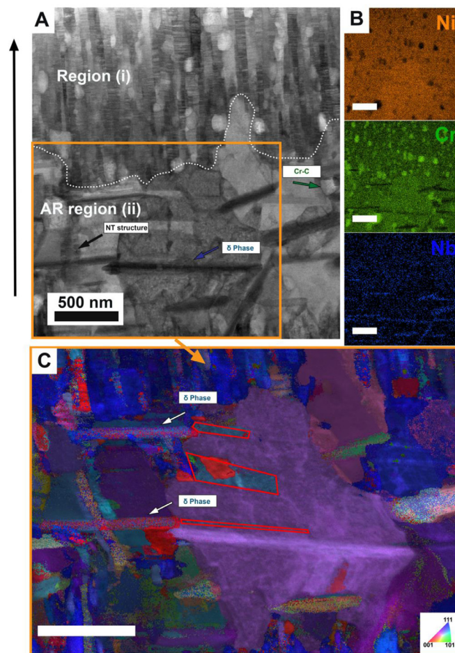
Fig. 7. (A) BF-STEM Image, corresponding (B) EDS maps of Ni, Cr, Nb, and (C) ACOM maps from the outlined (orange) region in (A) with inset of IPF triangle of the 8-hour aged sample. White scale bars are 500 nm.
