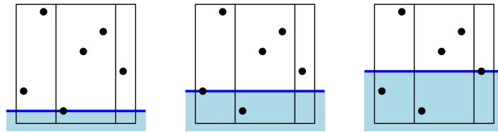
Figure 2. The scanline mapping allows us to encode permutations by words: above, the permutation \pi = 261453 is encoded by the word w(\pi) = 213221 (the sequence of runs encountered if one reads the permutation bottom-to-top).
