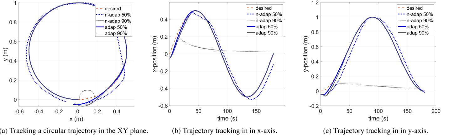
FIGURE 5: Comparison between the adaptive approach ( adap ) and the non-adaptive SAP controller ( n-adap ) for trajectory tracking using a tail-actuated robotic fish. The percentage indicates the deviation of the model parameters from their true values. For the adaptive controller, this indicates the initial deviation of the parameter estimates from their true values.
