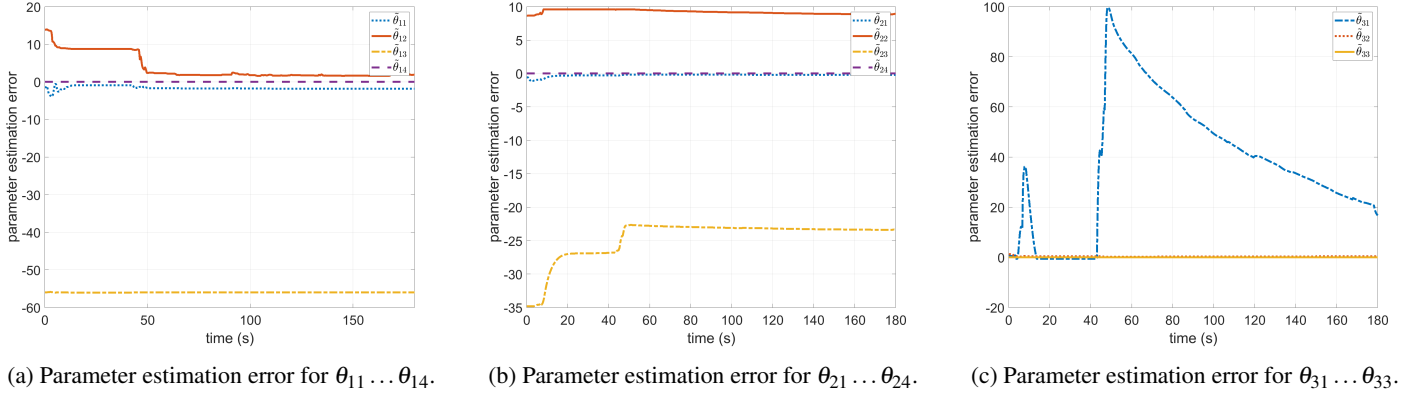
FIGURE 6: Error in parameter estimation for the tail-actuated robotic fish for the case where the parameters were initialized with \pm 90\% of their true values.
