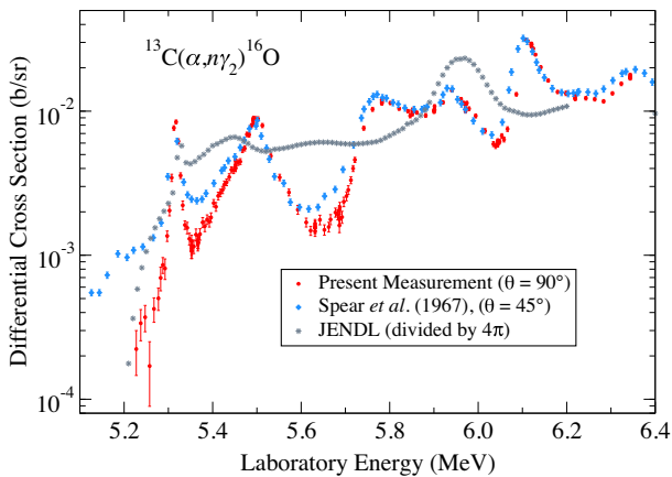
FIG. 2. Comparison of the ^{13}\text{C}(\alpha, n)^{16}\text{O} cross section measured at \theta_{\text{lab}} = 90^\circ (this Letter, red circles) and \theta_{\text{lab}} = 45^\circ (Spear et al. [40], open blue diamonds) to the angle integrated cross section evaluation of JENDL/AN-2005 [22] (gray line) scaled down by a factor of 4\pi .
