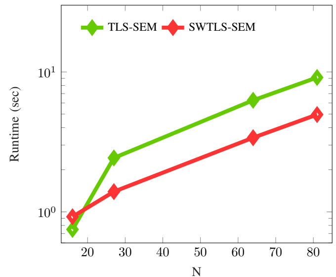
Figure 9: Runtime in seconds versus N .
