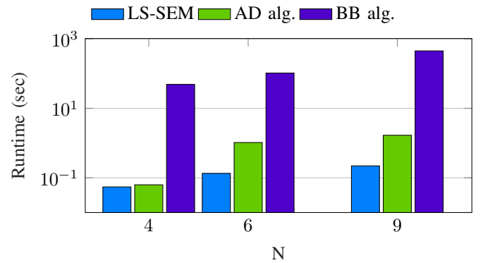
Figure 2: Runtime in seconds.
