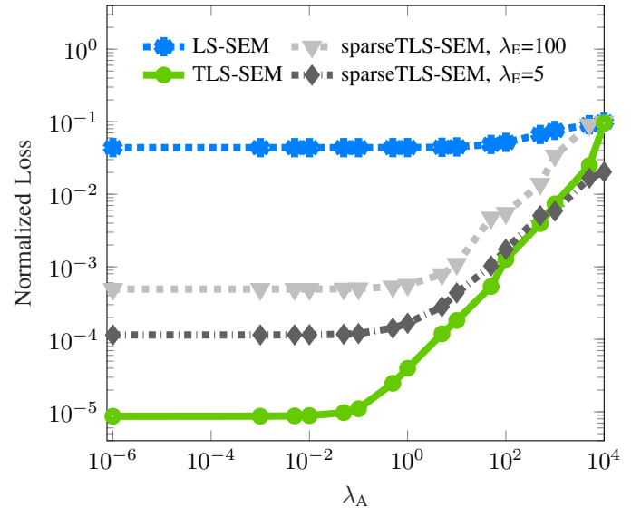
Figure 6: Loss function vs. \lambda_A for Gene regulatory network.
