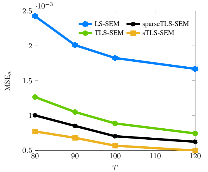
Figure 5: MSE_A as a function of T .
