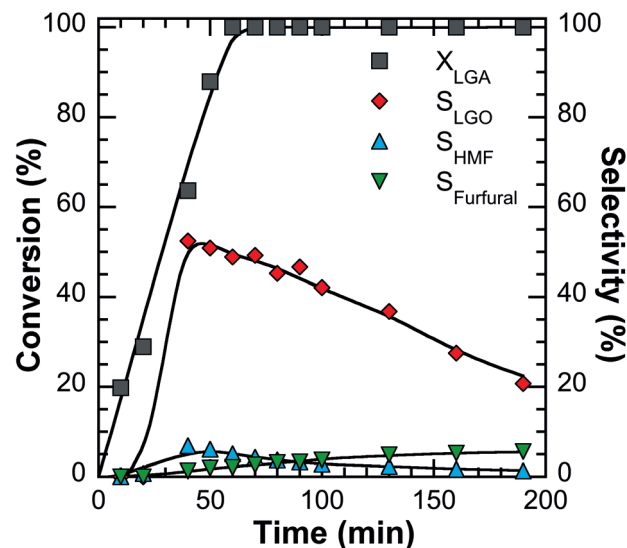
Fig. 5 Dehydration of 14 mM LGA using non-endcapped SiliaBond®-PSA catalyst in THF at 483 K and 69 bar He with an acid loading of 0.08 mmol H + .
