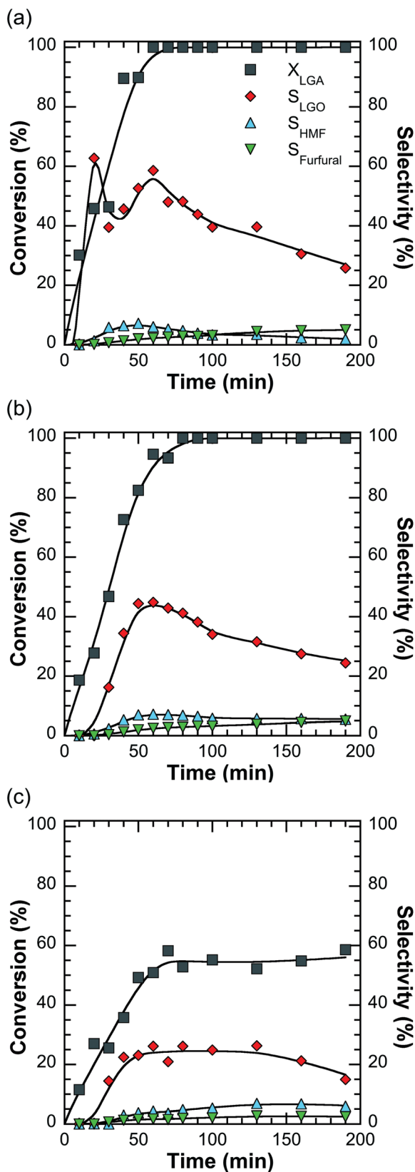
Fig. 6 Effect of LGA concentration on the dehydration of LGA using endcapped SiliaBond®-PSA catalyst in THF at 483 K and 69 bar He. The acid loading was kept at 0.08 mmol H^+ . The LGA concentrations were: (a) 14 mM, (b) 36 mM and (c) 89 mM.
