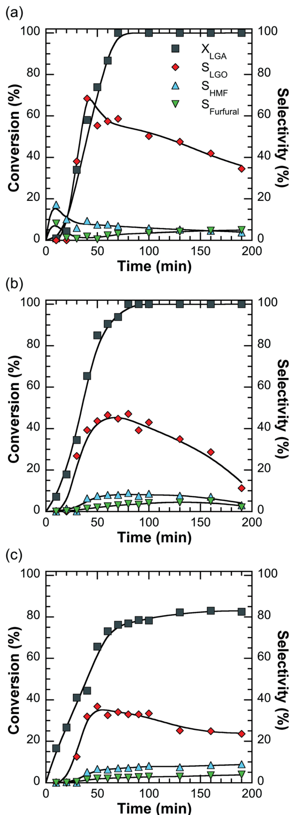
Fig. 3 Effect of LGA concentration on the dehydration of LGA using PS-SBA-15 catalyst in THF at 483 K and 69 bar He and LGA concentrations of (a) 14 mM, (b) 36 mM, and (c) 89 mM. The acid loading was kept to 0.08 mmol H^+ .
