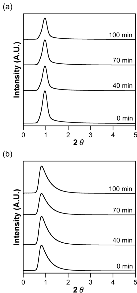
Fig. 9 Powder XRD pattern for functionalized silica with propyl sulfonic acid after thermal treatment in THF at 483 K: (a) PS-SBA-15 and (b) SiliaBond®-PSA endcapped.
