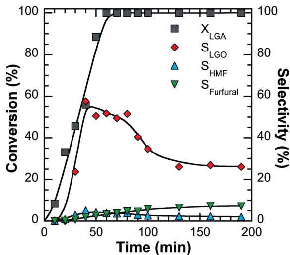
Fig. 8 Dehydration of 14 mM LGA using endcapped SiliaBond®-Tosic-a catalyst in THF at 483 K and 69 bar He with an acid loading of 0.08 mmol H + .
