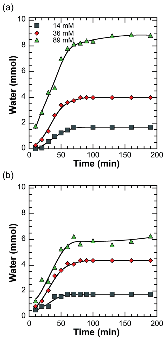
Fig. 4 Water production during the dehydration of LGA for different LGA initial concentrations in THF at 483 K and 69 bar He and catalysts: (a) PS-SBA-15 and (b) SiliaBond-PSA endcapped.
