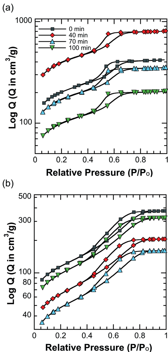
Fig. 10 \text{N}_2 adsorption and desorption isotherms for functionalized silica with propyl sulfonic acid after thermal treatment in THF at 483 K. Results for (a) PS-SBA-15 and (b) SiliaBond®-PSA endcapped.
