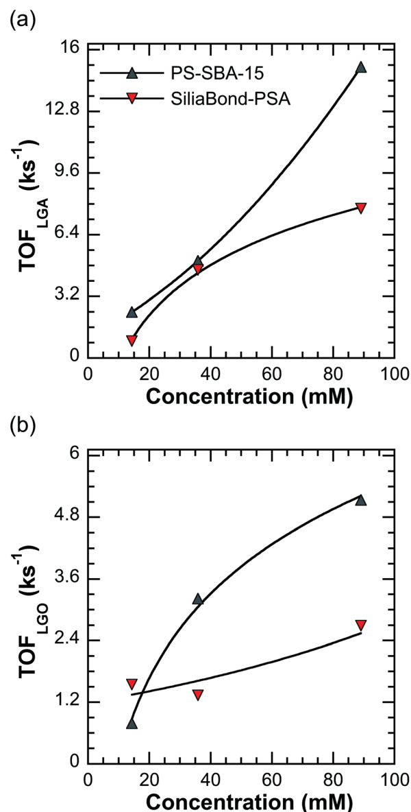
Fig. 7 Effect of LGA concentration on average TOF (a) of LGA consumption and (b) of LGO production using PS-SBA-15 and SiliaBond®-PSA catalysts in THF at 483 K and 69 bar. The acid loading was kept at 0.08 mmol H^+ .
