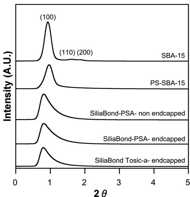
Fig. 1 Powder XRD patterns for silica catalysts functionalized with sulfonic acid groups.
