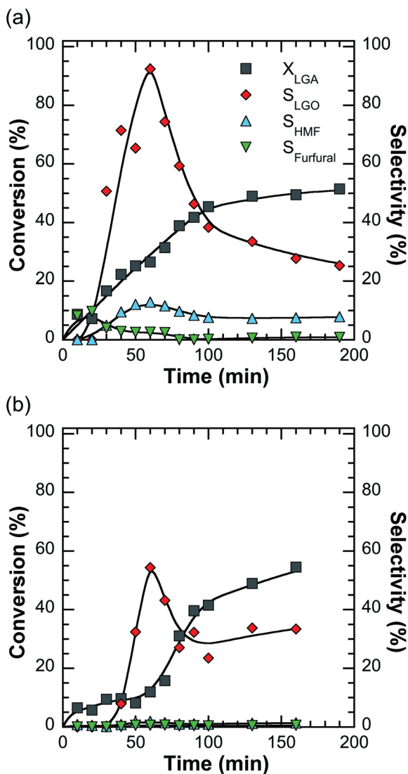
Fig. 2 Dehydration of 14 mM LGA using homogeneous acid catalysts: (a) \text{H}_2\text{SO}_4 and (b) 1-propanesulfonic acid in THF at 483 K and 69 bar He with 0.08 mmol \text{H}^+ .
