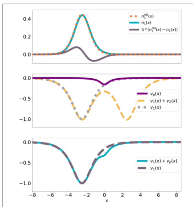
Figure 4. Graphic example of simplest PPT case for 2 non-interacting electrons in 1D potentials of the form v_{1,2}(x) = \cosh^2(x \pm a) , with a = 2.5 . Upper panel: The gray line magnifies the atomic-density distortion n_1(x) - n_1(x)^0 by a factor of 5 to highlight what occurs upon formation of the chemical bond: The density of the isolated atom is pulled towards the bonding region. Middle panel: Left atomic potential v_1(x) (dotted), total 'molecular potential' (dashed), and partition potential (solid, purple). Bottom panel: Comparison of the isolated atomic potential v_1(x) and the effective potential v_1(x) + v_p(x) for which the polarized density n_1(x) is a ground-state density.
