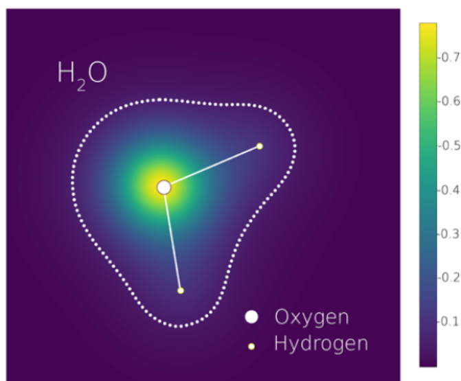
Figure 1. Ground state density of a water molecule on the plane of the three atoms. Calculated using Psi4 ( Smith, et al., 2018 ) ( Parrish, et al., 2017 ) with CCSD(T)/UGBS. The dotted line indicates a density iso-contour.
