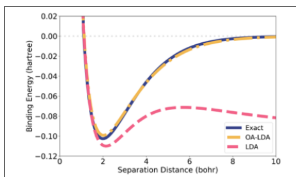
Figure 2. Electronic binding energy of H_2^+ . Exact (solid, blue), KS-LDA (dashed, pink), and OA-LDA (dash-dotted, yellow) from (Nafziger, 2015), as explained in Sec.IV.
