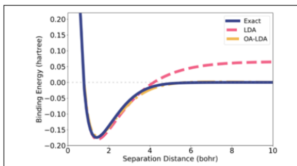
Figure 3. Electronic binding energy of H_2 . Exact (solid, blue), KS-LDA (dashed, pink), and OA-LDA (dash-dotted, yellow) from (Nafziger&Wasserman, 2015), as explained in Sec.IV.
