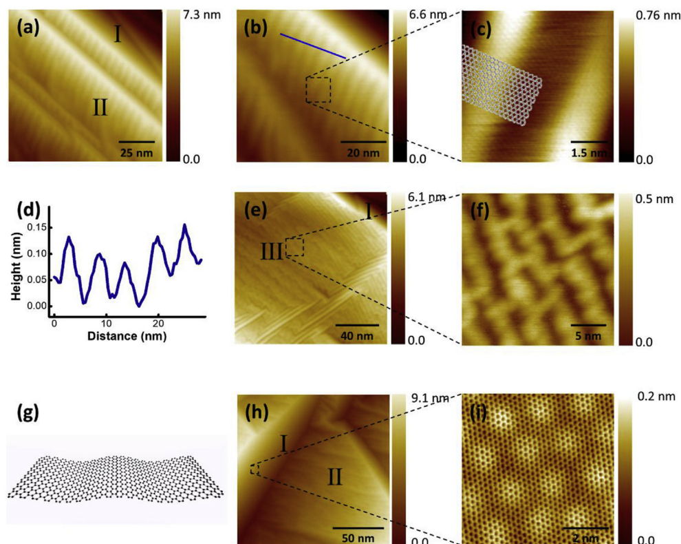
Fig. 1. (Color online) STM topographical images of planar graphene (labeled as I), 1D-rippled graphene (II) and 2D-rippled graphene (III) on Cu. (a) Large area STM image of planar graphene (I) and 1D-rippled graphene (II) showing the linear periodic modulation and the spatial modulation frequencies ( V_s = -2.340 V, I = 0.110 nA). (b) High-resolution STM image of 1D-rippled graphene ( V_s = -0.340 V, I = 1.900 nA). (c) STM image of the 1D-rippled graphene, observed from the square region marked in (b), the schematic model on top of the atomic image shows the ripples along zigzag direction ( V_s = -0.280 V, I = 1.900 nA). (d) Line profile perpendicular to the 1D-rippled graphene (marked as a blue line in (b)) showing the periodic modulation. (e) STM image of graphene on two different Cu facets, planar graphene (I) and 2D-rippled graphene (III) ( V_s = -2.74 V, I = 0.045 nA). (f) High-resolution STM image of 2D-rippled graphene, observed from the dashed square region marked in (e) ( V_s = -2.600 V, I = 0.068 nA). (g) A schematic model shows 1D-rippled graphene sheet. (h) Large area STM image of planar graphene (I) and 1D-rippled graphene (II) ( V_s = -1.850 V, I = 0.340 nA). (i) Atomic STM image showing the moiré pattern of planar graphene, observed from the dashed squared region marked in (h) ( V_s = -1.850 V, I = 0.450 nA).
