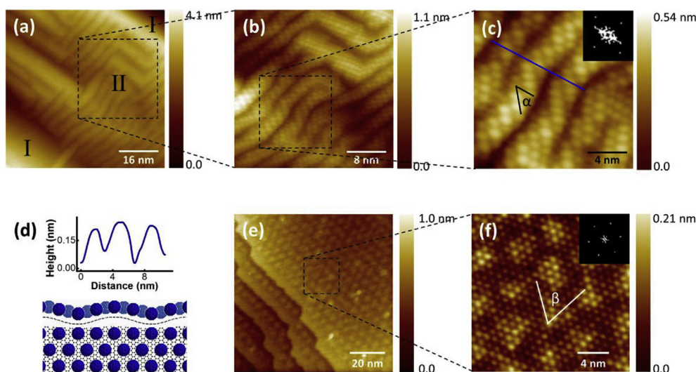
Fig. 2. (Color online) STM images of C_{60} on 1D-rippled graphene (II) and on planar graphene (I). (a) Large area STM topographic image of the C_{60} on 1D-rippled graphene showing well-defined linear periodic modulated ripple ( V_s = -2.00 V, I = 0.060 nA). (b) Zoomed-in STM image (measured from the dashed square of (a)) of C_{60} on a long periodic graphene ripple ( V_s = -2.60 V, I = 0.050 nA). (c) High-resolution image (measured from the dashed square region of (b)) C_{60} on 1D-rippled graphene, shows a lattice angle \alpha of 54.1^\circ with a quasi-hcp pattern ( V_s = -2.60 V, I = 0.040 nA). Inset, the corresponding FFT image of (c). (d) A line profile along the perpendicular direction of the 1D-rippled graphene marked with the blue line in (c) (top), side view and top view showing the quasi-hcp C_{60} on 1D-rippled graphene (bottom). (e) Large area STM image of the C_{60} on planar graphene with a well-defined moiré pattern on facet I ( V_s = -2.65 V, I = 0.046 nA). (f) High-resolution STM image of C_{60} on planar graphene (measured from the square region of (e)), showing a lattice angle \beta of 60.0^\circ and a moiré pattern. Inset, the corresponding FFT image of (f).
