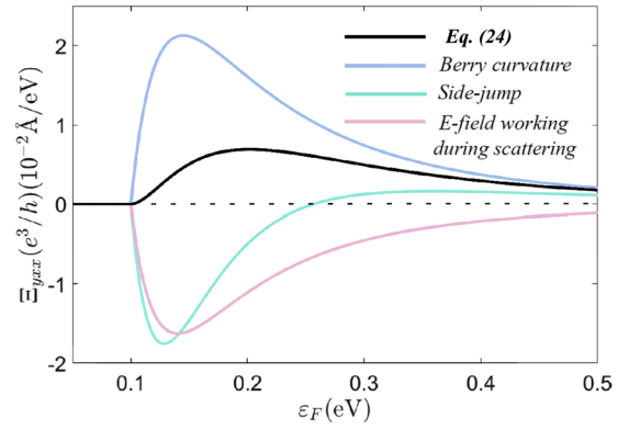
FIG. 2. The second-order nonlinear Hall responses in the 2D tilted massive Dirac model that are beyond the conventional Boltzmann equation, from the Berry curvature and side-jump velocities, the \mathbf{E} field working during scattering e\mathbf{E} \cdot \delta \mathbf{r}_{l'l} , and the interband effect of the \mathbf{E} field during scattering [Eq. (24)]. Parameters are chosen as t = 0.1 \text{ eV } \text{\AA} , v = 1 \text{ eV } \text{\AA} , \Delta = 0.1 \text{ eV} , n_i V_0^2 = 10^2 (\text{eV } \text{\AA})^2 . \hbar = 2\pi\hbar is the Planck constant.
