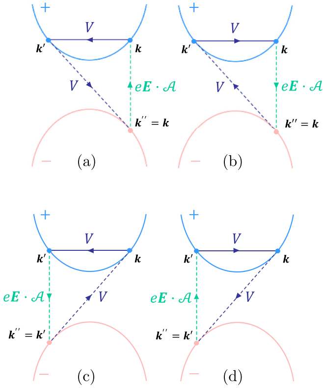
FIG. 1. Schematics of Eq. (9) describing the electric-field-induced interband virtual processes during scattering in two-band systems. The contributions from (a) and (b) to \delta^E W_{l'l} are complex conjugated, as are (c) and (d).
