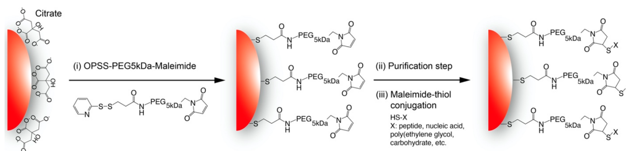
Figure 1. Schematic representation of maleimide-based nanoparticle surface functionalization. (i) OPSS-(PEG) 5kDa -Mal is conjugated to the surface of citrate-stabilized gold nanoparticles (depicted by red surface) via a ligand exchange reaction to form maleimide-functionalized nanoparticles. (ii) Maleimide-functionalized nanoparticles are then purified by centrifugation to remove excess OPSS-(PEG) 5kDa -Mal. (iii) Virtually any molecule with accessible thiol groups can then be conjugated to the nanoparticles via maleimide–thiol chemistry.
