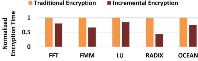
Figure 7: Encryption time comparison using traditional encryption and incremental encryption (our approach).
