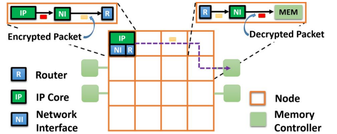
Figure 1: NoC based many-core architecture connecting IPs on a single SoC using a 4 \times 4 Mesh topology. Each node contains an IP that connects to a router via a network interface. Communication between two IPs (in this case, a processor IP and a memory controller) is encrypted so that an eavesdropper cannot extract the packet content.
