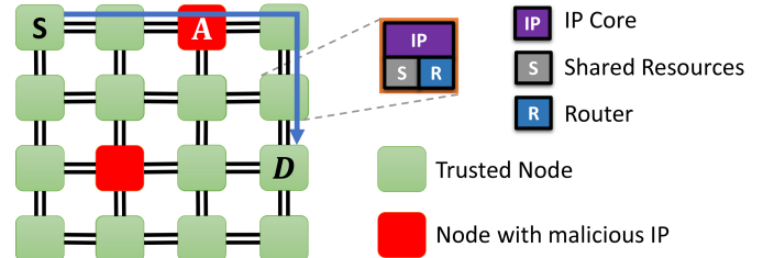
Fig. 1: A typical SoC architecture with a Mesh NoC.
