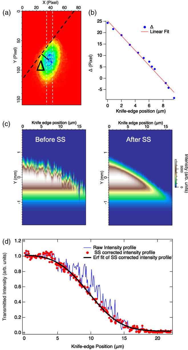
FIG. 4. Space-stamping to correct spatial jitter (a) typical knifed beam on detector, \Delta is defined as the distance between cut and Gaussian centroid. (b) Linear fit of \Delta using transmitted profiles with similar Gaussian centroids. (c) Intensity profile in the white dashed box region in (a) over the knife-edge scan without (left) and with (right) SS correction. (d) Comparison of the transmitted intensity profile with and without SS correction.
