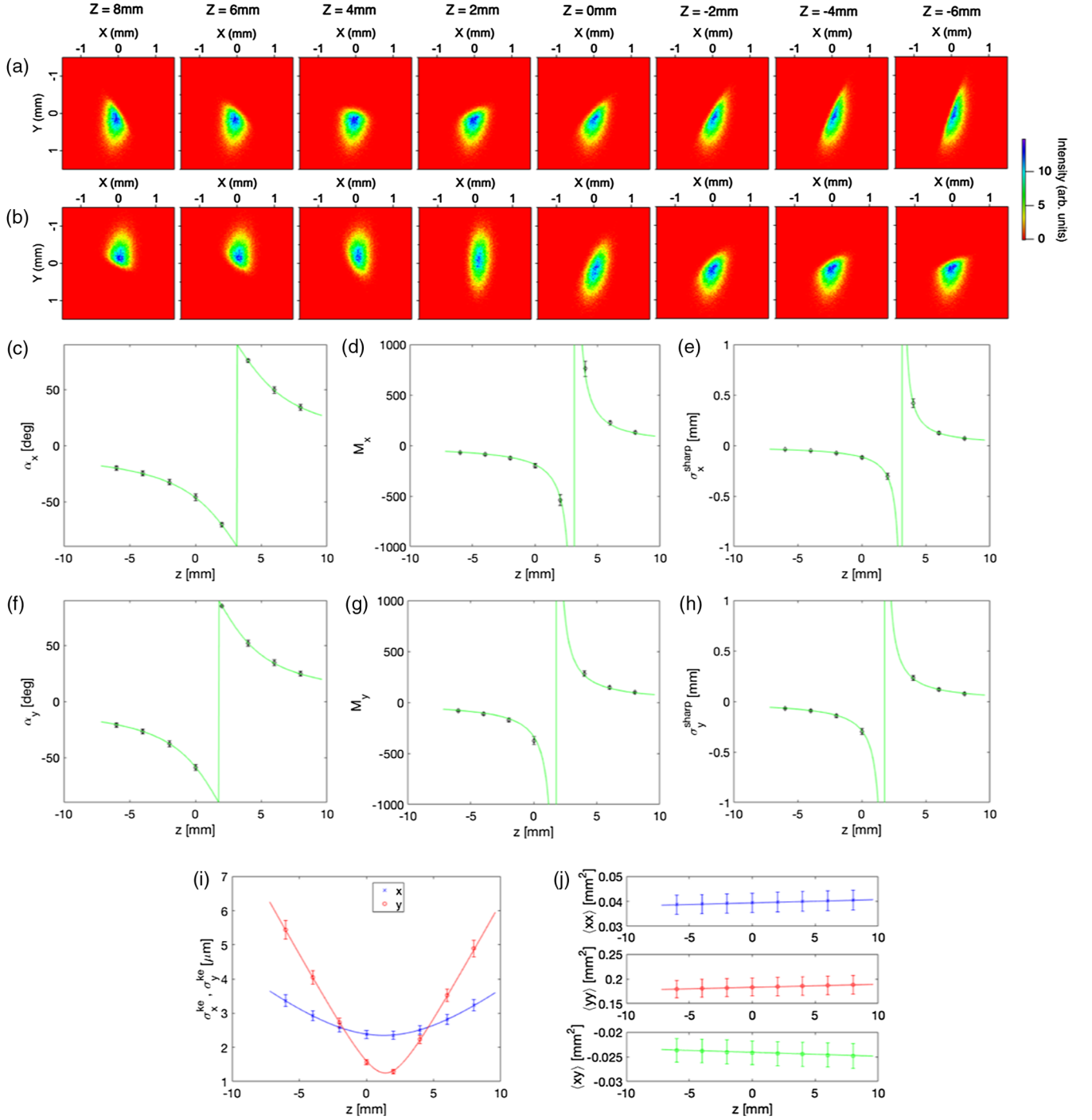
FIG. 2. Virtual measurement and its data analysis. (a)–(b) Simulated electron beam transverse shape at the detector screen after intercepting a vertical (a) and horizontal (b) semi-infinite plane, for different longitudinal positions of the plane. The (x, y) planes are coupled. (c)–(h) Example of curve fitting of virtual data: cut angle (c), (f), magnification (d), (g), and cut width (e), (h); (i)–(j) rms beam sizes at the knife-edge (i) and the detector (j).
