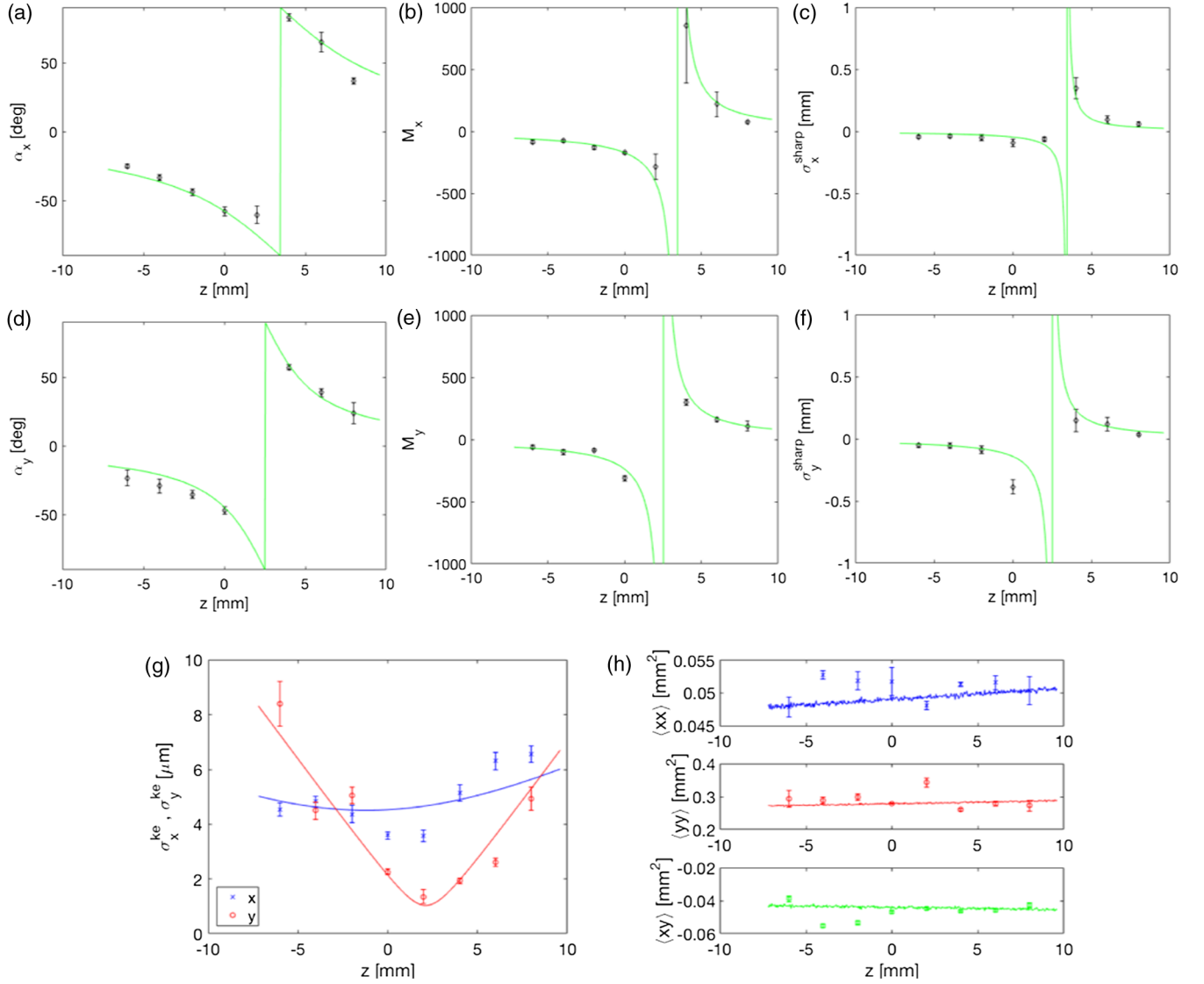
FIG. 5. Results of the global fitting to the measured data: cut angle (a), (d), magnification (b), (e), and cut width (c), (f); rms beam sizes at the knife-edge (g) and the detector (h).
