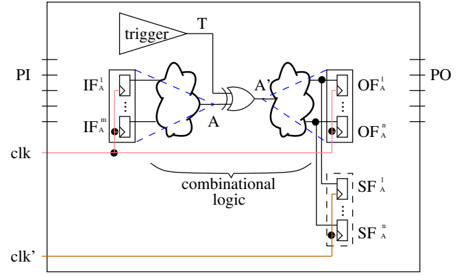
Fig. 2. Path delay measurement using shadow registers [34]. The registers of the input layer and the output layer of the asset A are represented using IF_A^i and OF_A^j , respectively. The path delay is measured by tuning clk' and comparing the values in the corresponding register of the output layer and the shadow registers, e.g., OF_A^i and SF_A^i .
