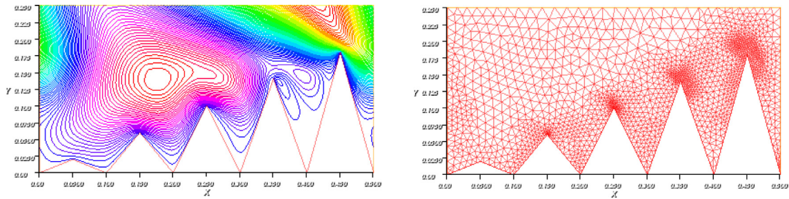
Fig. 4. The numerical solution of Example 2. (left) The contour plot of the magnitude of the solution; (right) The corresponding adaptively refined mesh.
