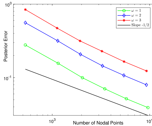
Fig. 3. Quasi-optimality of the a posteriori error estimates for Example 2.
