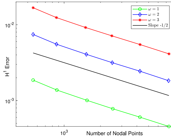
Fig. 2. Quasi-optimality of the a priori error estimates for Example 1.
