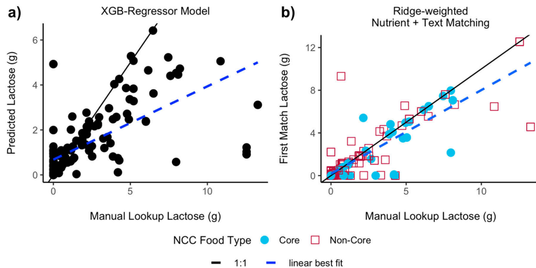
Figure 3. Comparison of the lactose (g) from the manual lookup to the (a) prediction from the XGB-Regressor model and (b) the Ridge-weighted Nutrient + Text database matching. For (b), markers are colored according to whether the first match was an NCC core food or a non-core food. Example of core foods are apples, honey, and bread. Examples of non-core foods are Genoa salami, cheese bread, and scrambled eggs.
