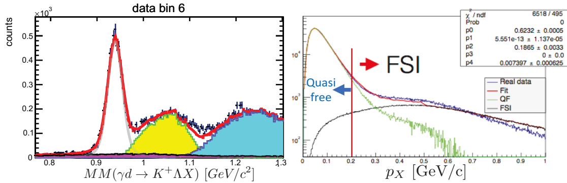
Figure 4: Left: Missing-mass distribution of \gamma d \rightarrow K^+ \Lambda X indicated the various sources of background ( \Sigma channel with yellow, \Sigma^* channel with cyan, and accidentals with magenta). Right: Missing momentum of the reaction indicating the typical cut applied to select quasi-free or FSI- dominated samples.
