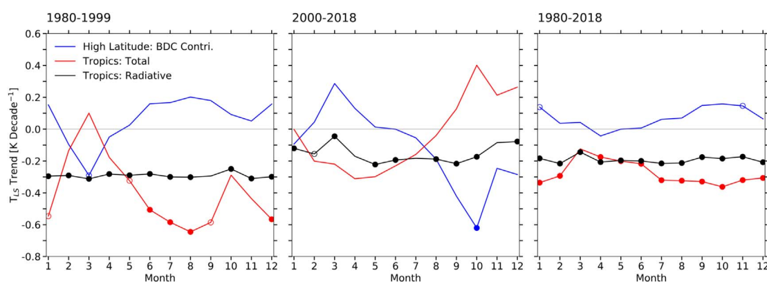
Figure 3. The lower-stratospheric temperature ( T_{LS} ) trends due to changes of the Brewer–Dobson circulation (BDC) over combined high latitudes ( 40^{\circ}\text{N} – 82.5^{\circ}\text{N} and 40^{\circ}\text{S} – 82.5^{\circ}\text{S} ) (blue lines) and MSU/AMSU-observed T_{LS} trends in the tropics ( 20^{\circ}\text{N} – 20^{\circ}\text{S} ) (red lines) along with its estimated radiative component (black lines), versus month, for 1980–1999 (left), 2000–2018 (middle), and 1980–2018 (right). The trends are shown as filled (open) circles when they are significant at the 95% (90%) confidence levels.
