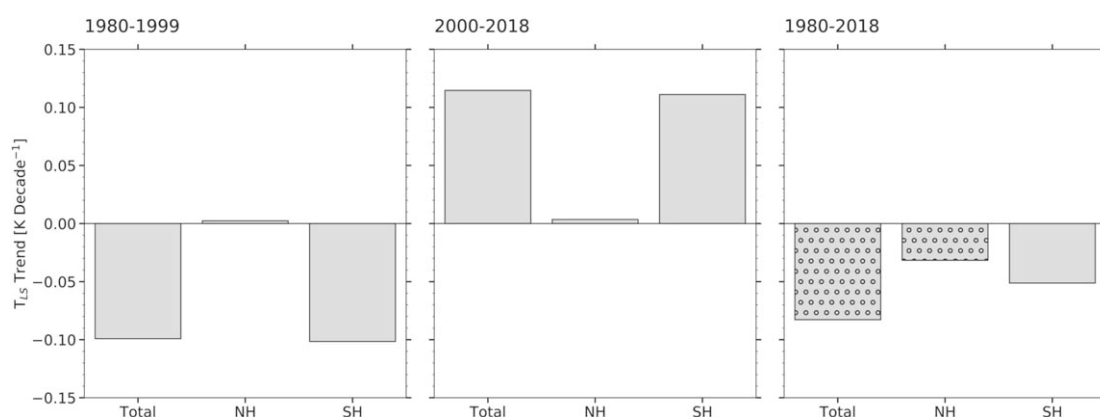
Figure 4. Annual mean lower-stratospheric temperature ( T_{LS} ) trend in the tropics ( 20^{\circ}\text{N} – 20^{\circ}\text{S} ) due to changes of the BDC and the contribution from the Northern Hemisphere (NH) and Southern Hemisphere (SH) cells for 1980–1999 (left), 2000–2018 (middle), and 1980–2018 (right). The trend bars marked with open circles are significant at the 90% confidence levels.
