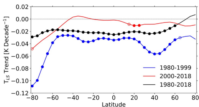
Figure 2. Lower-stratospheric temperature ( T_{LS} ) trend as a function of latitude based on zonal-mean T_{LS} temperature anomaly time series for 1980–1999 (blue), 2000–2018 (red), and 1980–2018 (black) from MSU/AMSU observations. The trends are shown as filled (open) circles when they are significant at the 95% (90%) confidence levels.
