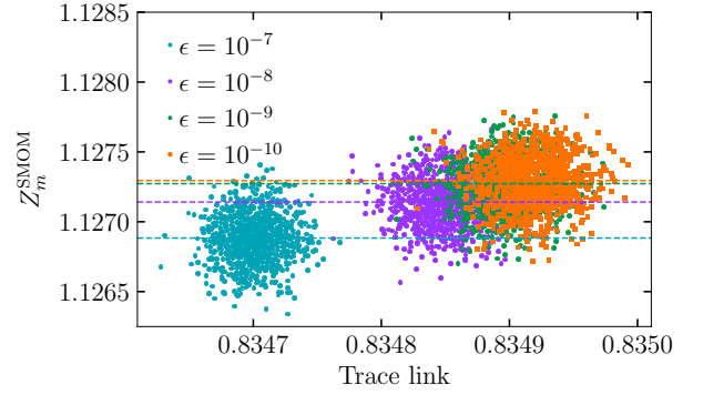
FIG. 1: Scatter plots from bootstrap samples of Z_m^{\text{SMOM}} at \mu = 2 GeV and Landau gauge Trace link values on coarse set 4, for a quark mass value in lattice units of 0.0153. On the left results are for a gauge-fixing tolerance on 10^{-7} (the tolerance we use); on the right the tolerance is successively tightened to 10^{-10} . Mean values for Z_m^{\text{SMOM}} are indicated by dashed lines of matching colour.
