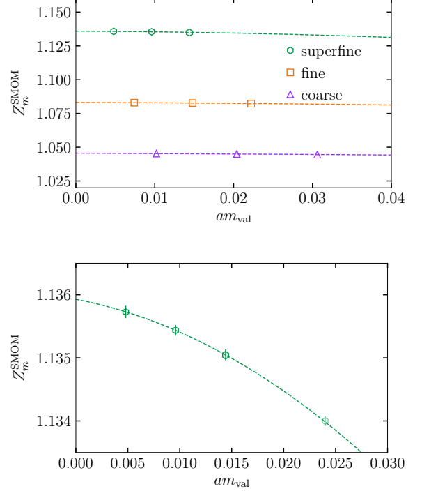
FIG. 7: The upper plot shows the dependence of Z_m^{\text{SMOM}} on valence quark mass in lattice units for coarse, fine and superfine lattices (sets 2, 10 and 12) at \mu = 3 GeV. The dashed line gives the simple fit described in the text. The lower plot is a zoomed in version of the superfine (set 12) results for which fit parameters are shown in Figure 8. The lighter rightmost point corresponds to a quark mass equal to that of the strange quark. This point was not included in the valence quark mass fit, but lies on top of the fitted line.
