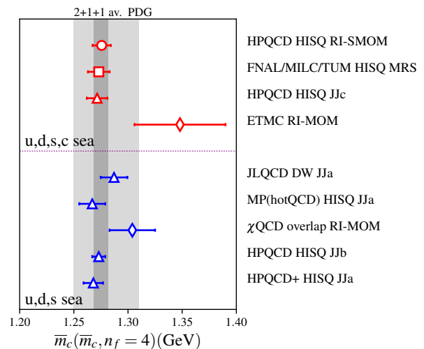
FIG. 12: Comparison of lattice QCD results for \overline{m}_c(\overline{m}_c, n_f = 4) . Note that results are determined at a higher energy scale and then run down to \overline{m}_c using perturbation theory. Calculations are listed chronologically and divided into those obtained on gluon configurations that include 3 (blue symbol) or 4 (red symbol) flavours of quarks in the sea. Results obtained on 3 flavour configurations have in all cases been adjusted to n_f = 4 using perturbation theory (see the references for details of how this is done in each case). Different symbols denote different methods: open triangles, the current-current correlator (JJ) method ('a', 'b' and 'c' variants, see text); open diamonds use the RI-MOM intermediate scheme, open circles, the RI-SMOM intermediate scheme and open squares, the MRS scheme. Labels on the right indicate collaboration name, quark formalism and method. The result denoted 'HPQCD HISQ RI-SMOM' is this work, 'FNAL/MILC/TUM HISQ MRS' is from [22], 'HPQCD HISQ JJ' (red) is from [12], 'ETMC RI-MOM' is from [20], 'JLQCD DW JJ' is from [15], 'MP(hotQCD) HISQ JJ' is from [16], 'chiQCD overlap RI-MOM' is from [65], 'HPQCD HISQ JJ' (blue) is from [13] and 'HPQCD+ HISQ JJ' is from [4]. The grey shaded band indicates the world average (taking correlations into account) of the n_f = 4 results and the lighter shaded band shows the evaluation of 1.28(3) GeV from the Particle Data Group [66].
