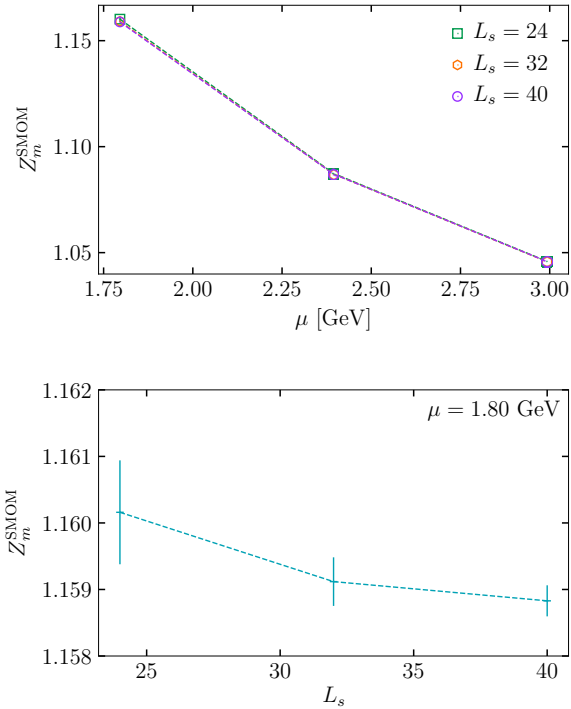
FIG. 9: Dependence of Z_m^{\text{SMOM}} on the spatial volume of the lattice (sets 3, 4 and 5) as a function of \mu . The valence quark mass in lattice units is fixed to 0.0051.
