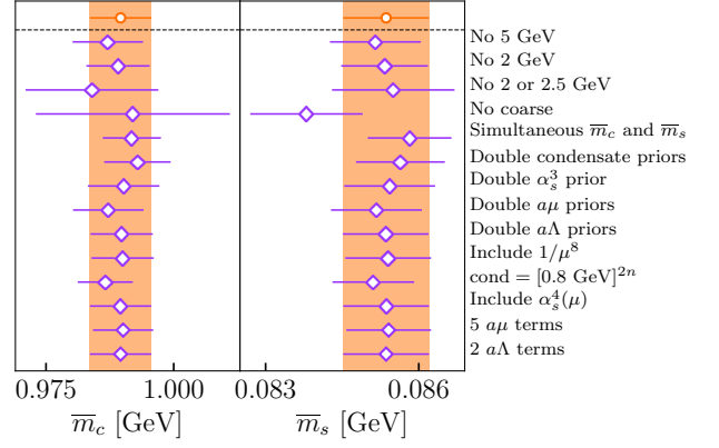
FIG. 11: A graphical representation of the different tests that we have done to check the robustness of our fits to obtain the physical results for \overline{m}_s and \overline{m}_c . The different rows give variations on the fit described in the text (eq. (26)).
