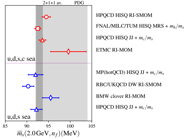
FIG. 13: Comparison of lattice QCD results for \bar{m}_s(2.0 \text{ GeV}, n_f) . Results are listed chronologically and divided into those obtained on gluon configurations that include n_f = 3 (blue symbol) or n_f = 4 (red symbol) flavours of quarks in the sea. The n_f = 4 results should be 0.2 MeV smaller than n_f = 3 from QCD perturbation theory matching for adding/removing a c sea quark. Different symbols denote different methods: open triangles, the current-current correlator (JJ) method combined with a nonperturbative determination of m_c/m_s ; open diamonds use the RI-MOM intermediate scheme and open circles, the RI-SMOM intermediate scheme and open squares the MRS scheme combined with a nonperturbative determination of a mass ratio between heavy and s quarks. Labels on the right indicate collaboration name, quark formalism and method. The result denoted ‘HPQCD HISQ RI-SMOM’ is this work, ‘FNAL/MILC/TUM HISQ MRS + m_h/m_s ’ is from [22], ‘HPQCD HISQ JJ + m_c/m_s ’ (red) is from [12], ‘ETMC RI-MOM’ is from [20], ‘MP(hotQCD) HISQ JJ + m_c/m_s ’ is from [16], ‘RBC/UKQCD DW RI-SMOM’ is from [67] (note that this uses a different method to fix Z_q than is used here), ‘BMW clover RI-MOM’ is from [68, 69], ‘HPQCD HISQ JJ + m_c/m_s ’ (blue) is from [13, 17]. The light grey shaded band shows the evaluation of 96(+8, -4) \text{ GeV} from the Particle Data Group [66]. The dark grey shaded band gives the weighted average (allowing for correlations) of the n_f = 2 + 1 + 1 results as described in the text.
