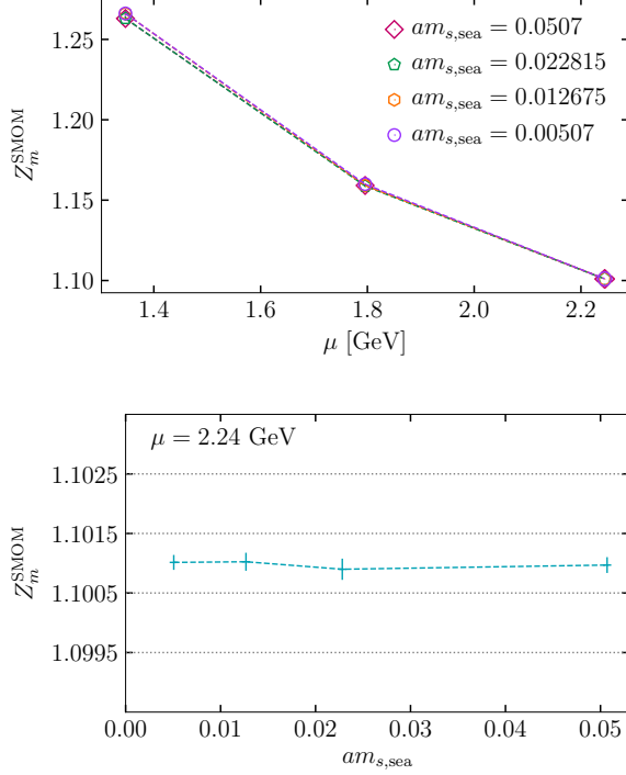
FIG. 4: Results for Z_m^{\text{SMOM}} for coarse ensembles with different values of the sea s quark mass, with u/d and c sea quark masses fixed in lattice units at 0.00507 and 0.628 respectively (sets 4, 6, 7 and 8, see Table II). The upper plot shows results for Z_m^{\text{SMOM}} as a function of \mu in GeV for the four sets. Dashed lines join the points. In all cases the valence quark mass is set to 0.0051 in lattice units. The lower plot gives more detail for results at \mu = 2.24 GeV, showing no visible variation (using the horizontal dotted lines as guides) in Z_m^{\text{SMOM}} even at a level below 0.1%.
