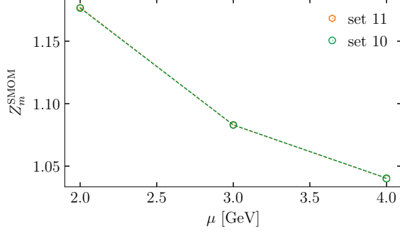
FIG. 6: Results for Z_m^{\text{SMOM}} for fine ensembles with different values of the sea u/d quark mass from sets 10 and 11 (see Table II). These sets also have slightly different s and c sea quark masses and spatial volume. The plot shows results for Z_m^{\text{SMOM}} as a function of \mu in GeV for the two sets, for a valence mass in lattice units of 0.0074.
