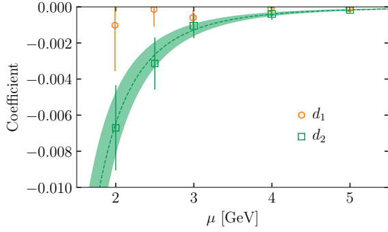
FIG. 8: The linear and quadratic slopes ( d_1 and d_2 of eq. (19)) of Z_m^{\text{SMOM}} with valence quark mass on superfine lattices (set 12), plotted against \mu in GeV. The curve with error band is a fit to the form C/\mu^4 through the d_2 points.
