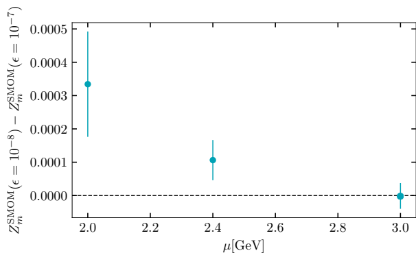
FIG. 2: The impact of the gauge fixing tolerance on Z_m^{\text{SMOM}}(\mu) as a function of \mu . Results are for coarse set 2, for a quark mass in lattice units of 0.0204, and show a steep fall with value of \mu consistent with sensitivity to gauge-noninvariant condensates.
