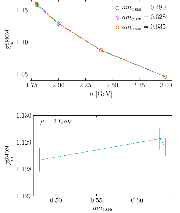
FIG. 5: Results for Z_m^{\text{SMOM}} for coarse ensembles with different values of the sea c quark mass from sets 1, 2 and 3 (see Table II). These sets have slightly different u/d and s sea quark masses, but by an amount which is much smaller than the change in the c sea mass from set 1 to sets 2 and 3. The upper plot shows results for Z_m^{\text{SMOM}} as a function of \mu in GeV for the two sets. The results shown here are obtained for a valence quark mass in lattice units of 0.0051. The lower plot shows more detail for results at \mu = 2.4 GeV, showing \mathcal{O}(0.1\%) variation for a very substantial change in am_{c,\text{sea}} . Dashed lines simply join the points.
