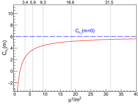
FIG. 14: The coefficient C_{n_f} which enters the Z_m^{\overline{\text{MS}}/\text{SMOM}} factor at \mathcal{O}(\alpha_s^2) as a function of \mu^2/m^2 for a massive sea quark of mass m . The dashed, blue line shows the m = 0 result. The solid, red line shows the exact result of a numerical evaluation of the contribution which is valid across the full range of m values. The vertical lines denote the location of the different \mu^2/m^2 values, which are used in this section.
