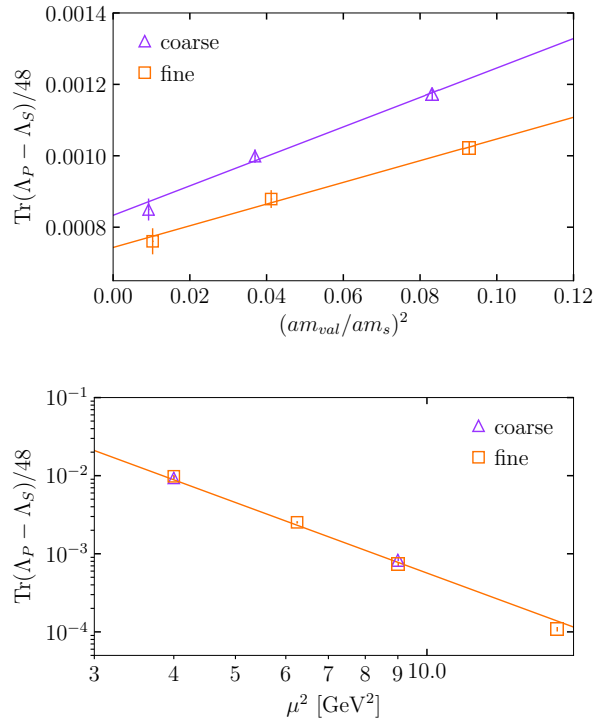
FIG. 3: The difference of vertex functions \Lambda_P and \Lambda_S (proportional to Z_P - Z_S ) as a function of valence quark mass and as a function of \mu . Upper plot: \text{Tr}(\Lambda_P - \Lambda_S)/48 at \mu = 3 GeV plotted against the square of the valence quark mass in units of the tuned s quark mass. Results are shown for coarse and fine lattices (sets 3 and 10). Lower plot: \text{Tr}(\Lambda_P - \Lambda_S)/48 extrapolated to zero valence quark mass, following the upper plot, now plotted against \mu on a log-log scale. For comparison, the line shows a constant divided by \mu^6 . This plot shows that, in the RI-SMOM scheme, the nonperturbative contributions to \Lambda_P - \Lambda_S are much more strongly suppressed than in the RI-MOM scheme, falling as \mu^{-6} .
