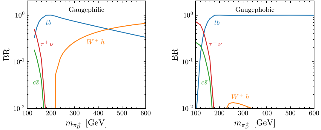
Figure 2. Branching ratios of the charged pions.
