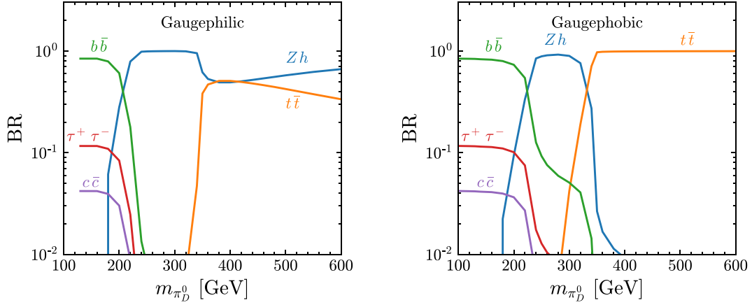
Figure 3. Branching ratios of the neutral pions.
