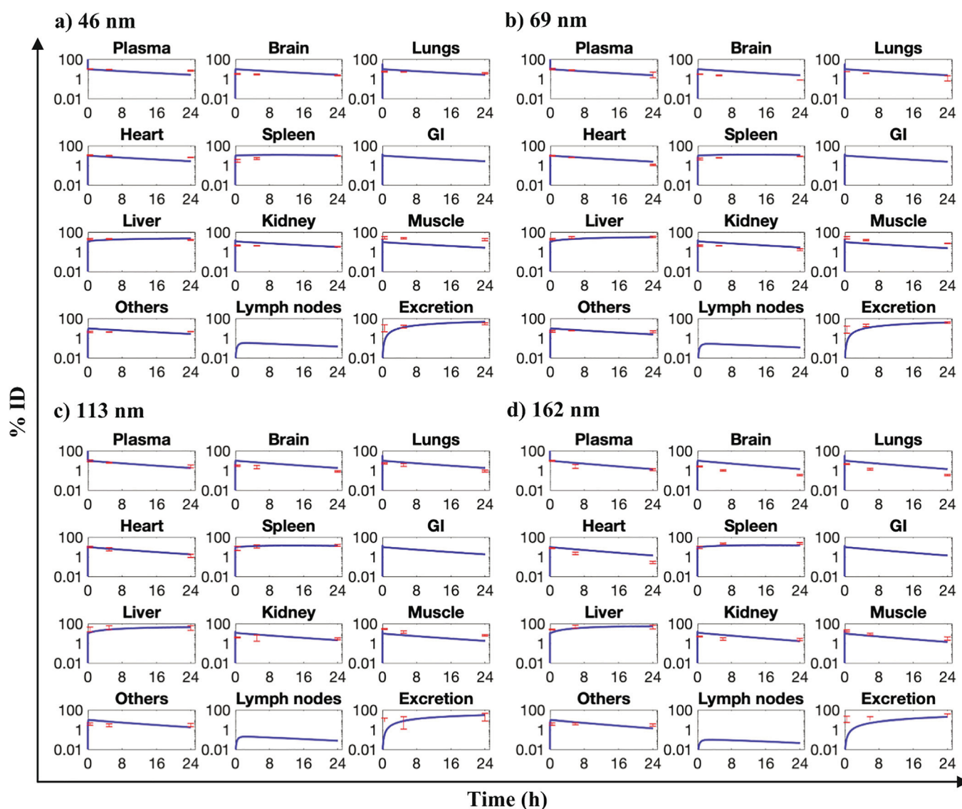
Fig. 2. In vivo model validation. Model simulation outputs for NPs of size a) 46 nm, b) 69 nm, c) 113 nm, and d) 162 nm are shown as blue lines in various model compartments. Red dots and error bars represent mean \pm S.D. of the experimental data from the literature for mesoporous silica NPs of matching hydrodynamic sizes ( n = 4 animals per group). Note: y-axes are in logarithmic scale. (For interpretation of the references to colour in this figure legend, the reader is referred to the web version of this article.)
