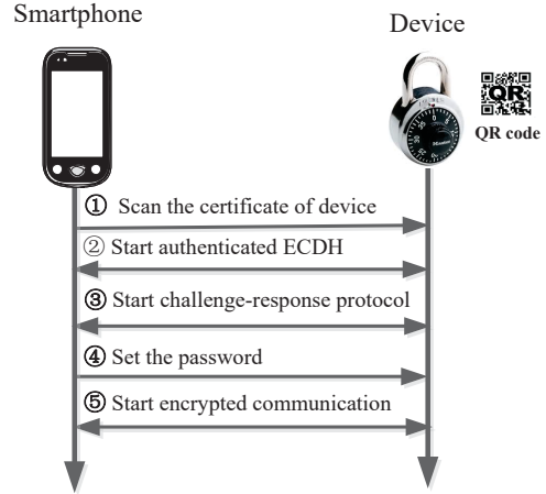
Fig. 2: The principle of our defense
