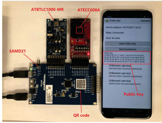
Fig. 1: The prototype of the application level defense
