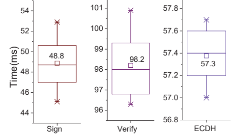
Fig. 8: Time for ECDSA/ECDH
