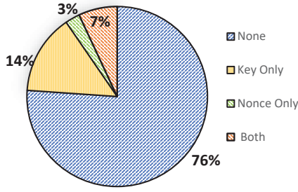
Fig. 3: Security State of BLE Products
