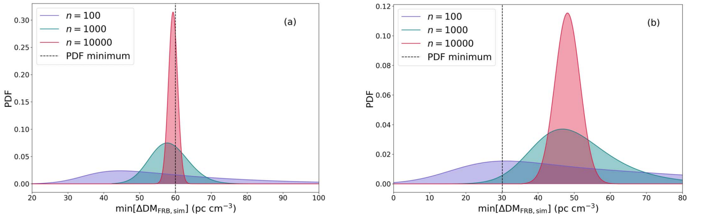
Figure A1. (a) \min[\Delta DM_{FRB}] with DM_{host} a delta function at 30 \text{ pc cm}^{-3} . The absolute minimum is 60 \text{ pc cm}^{-3} . (b) \min[\Delta DM_{FRB}] for a Gaussian DM_{host} with \mu = 60 \text{ pc cm}^{-3} and \sigma = 15 . The absolute minimum is 30 \text{ pc cm}^{-3} .
