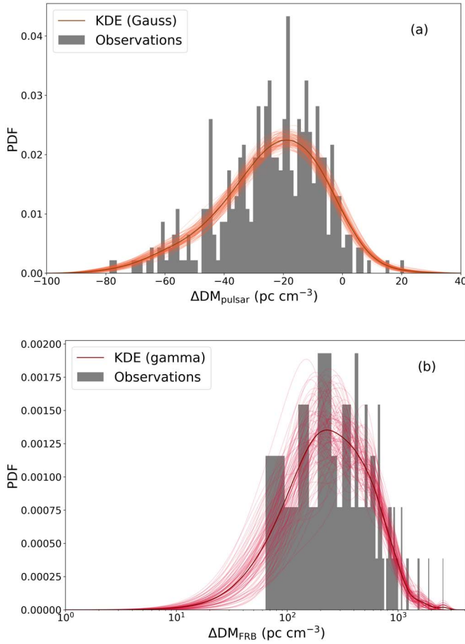
Figure 2. Distributions for observed samples, restricted to |b| > 20^\circ and using NE2001 for modeling \text{DM}_{\text{ISM}} . Overlaid on the data are PDFs derived with KDE. (a) \Delta\text{DM}_{\text{pulsar}} KDEs (with Gaussian kernels and a fixed bandwidth) overlaid on the observed data. The dark orange curve denotes the PDF estimated with the original data, and the lighter curves denote PDFs generated with resampled data. The bandwidth for each distribution is selected with cross-correlation and a search range between h = 8 and h = 15 . (b) \Delta\text{DM}_{\text{FRB}} KDEs (with gamma kernels and variable bandwidths) overlaid on the observed data. The thick dark-red curve denotes the PDF generated with the original data and the lighter curves denote PDFs generated with the resampled data.
