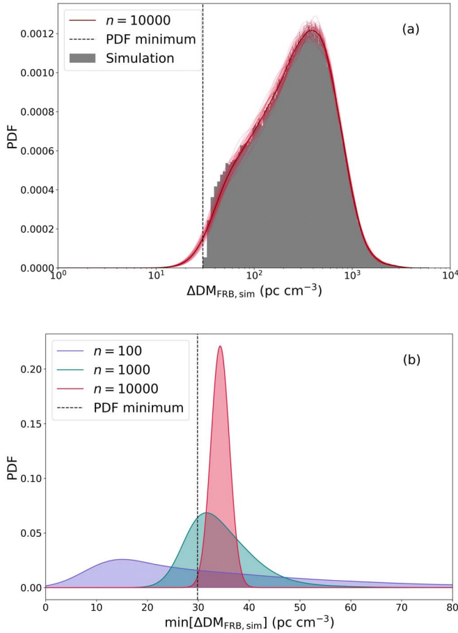
Figure 3. (a) Distribution of \Delta\text{DM}_{\text{FRB},\text{sim}} from simulated data. The KDE (gamma) estimation for n = 10,000 is denoted by the thicker dark-red line. The thinner red lines show the ensemble of KDEs from resampled data. (b) Distributions of \min[\Delta\text{DM}_{\text{FRB},\text{sim}}] given by the maximum gradients of the KDE (gamma) PDFs. As the sample size increases, solutions settle with higher certainty to \min[\Delta\text{DM}_{\text{FRB},\text{sim}}] = 34 \text{ pc cm}^{-3} , which is 4 \text{ pc cm}^{-3} above the absolute minimum.
