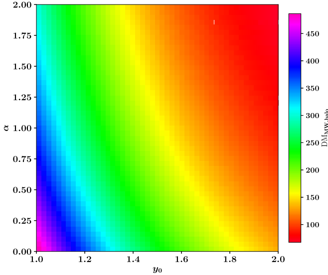
Figure 4. Predicted \text{DM}_{\text{MW,halo}} for our Galaxy as a function of two shape parameters that describe the assumed baryonic density profile (Prochaska & Zheng 2019). The analysis assumes a Galactic halo with total baryonic mass M_b \approx 2.4 \times 10^{11} M_\odot and that 75% of those baryons are in an ionized diffuse phase of the halo. The upper limit of \text{DM}_{\text{MW,halo}} < 123 \text{ pc cm}^{-3} rules out density profiles that more closely resemble the NFW profile ( \alpha = 0 , y_0 = 1 ).
