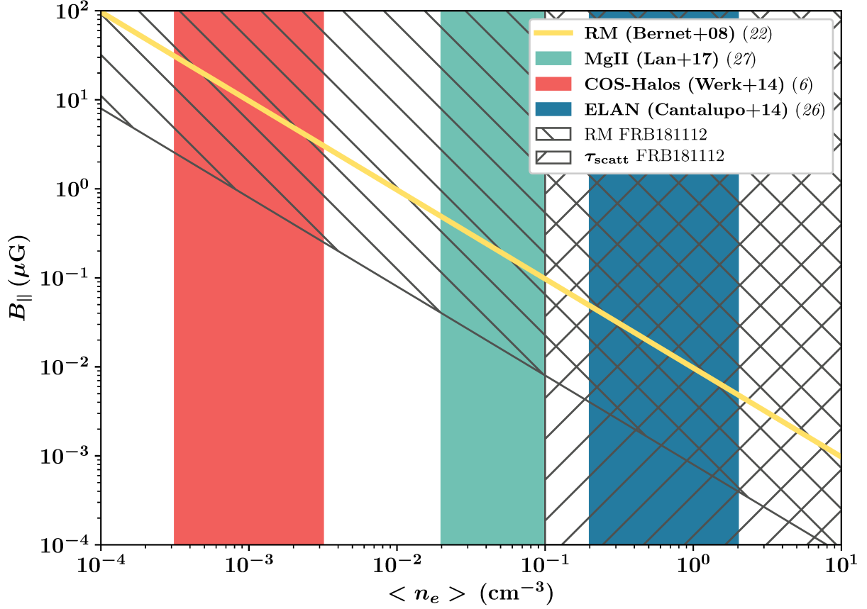
Figure 3: Constraints on the coherent magnetic field parallel to the line of sight B_{\parallel} and electron density n_e in the halo of FG-181112. The hatched regions show the parameter space in B_{\parallel} , n_e (cool gas) ruled out for the halo of FG-181112 from the measured RM and \tau_{\text{scatt}} of FRB 181112. These constraints are largely independent of the properties of the foreground galaxy. We compare these results with previous inferences for the density of cool halo gas (colored regions) based on ionization modeling and Ly \alpha fluorescence. We also illustrate previous estimations for the magnetic field strength in halo gas (yellow curve; (22)) which conflict with our results.
