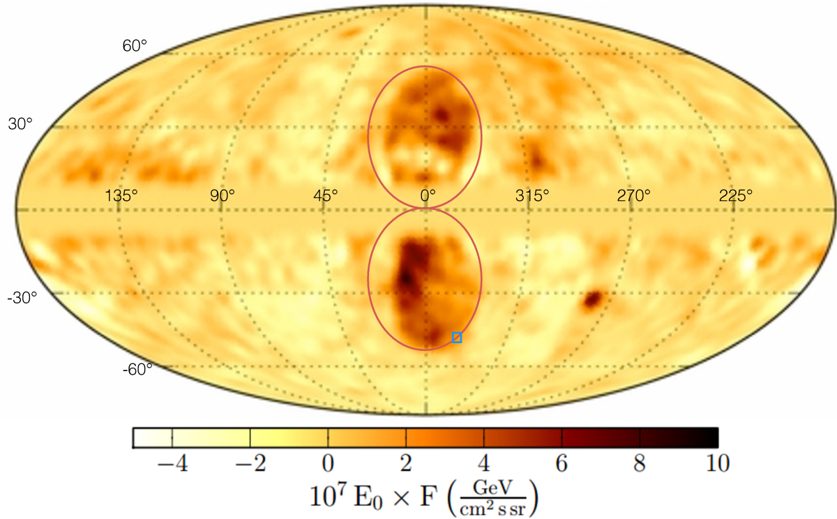
Fig. S11: The sightline to FRB 181112 intersects the southern Fermi bubble. The all-sky Fermi residual gamma-ray intensity map observed in the 3–10 GeV range, in Galactic coordinates centered on the Galactic Center (adapted from (68, 86)). The twin Fermi Bubbles are marked by the red ellipses. The blue square marks the line of sight through the Fermi Bubbles towards FRB 181112, which intersects the edge of the southern bubble.
