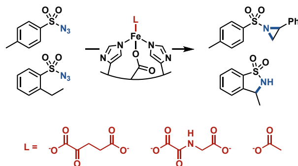
Figure 1. Small-molecule activation of a non-heme iron center for nitrene transfer. Carboxylate-containing ligands \alpha -ketoglutarate, N-oxalylglycine, and acetate modulate the nitrene-transfer activity of variants of P. savastanoi ethylene-forming enzyme.
