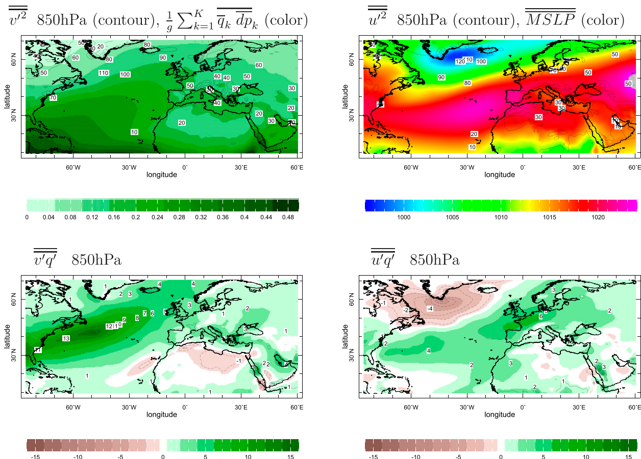
FIG. 3. Climatologies of quantities important to winter (DJFM) precipitation variability over 1979–2017 in the Atlantic–European–Mediterranean domain. (top left) The vertically integrated humidity (color shading; \text{kg m}^{-2} ) and 850-hPa transient eddy meridional velocity variance (contours; \text{m}^2 \text{s}^{-2} ). (top right) Mean sea level pressure (color shading; hPa) and the transient eddy zonal velocity variance (contours; \text{m}^2 \text{s}^{-2} ). Also shown are the climatological transient eddy (bottom left) meridional and (bottom right) zonal moisture flux at 850 hPa ( \text{m s}^{-1} ) times 1000.
