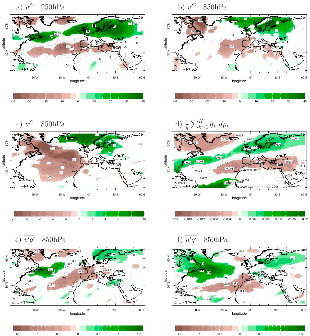
FIG. 5. For winter (DJFM) 1979–2017, regression on the NAO index of \overline{v'^2} ( \text{m}^2 \text{s}^{-2} ) at (a) 250 and (b) 850 hPa ( \text{m}^2 \text{s}^{-2} ), (c) \overline{u'^2} at 850 hPa ( \text{m}^2 \text{s}^{-2} ), (d) vertically integrated specific humidity ( \text{kg m}^{-2} ), and transient eddy moisture fluxes at 850 hPa in the (e) meridional and (f) zonal direction [ \text{kg (m s}^{-1}) ]. Color shading is added where the anomalies are significant at the 95% level according to a two-sided t test.
