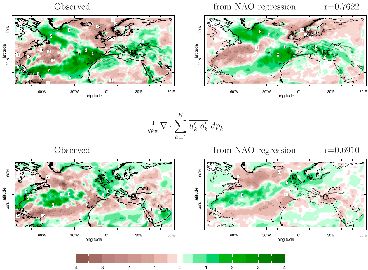
FIG. 10. As in Fig. 8, but for the extreme negative NAO winter (DJFM) of 2009/10.
