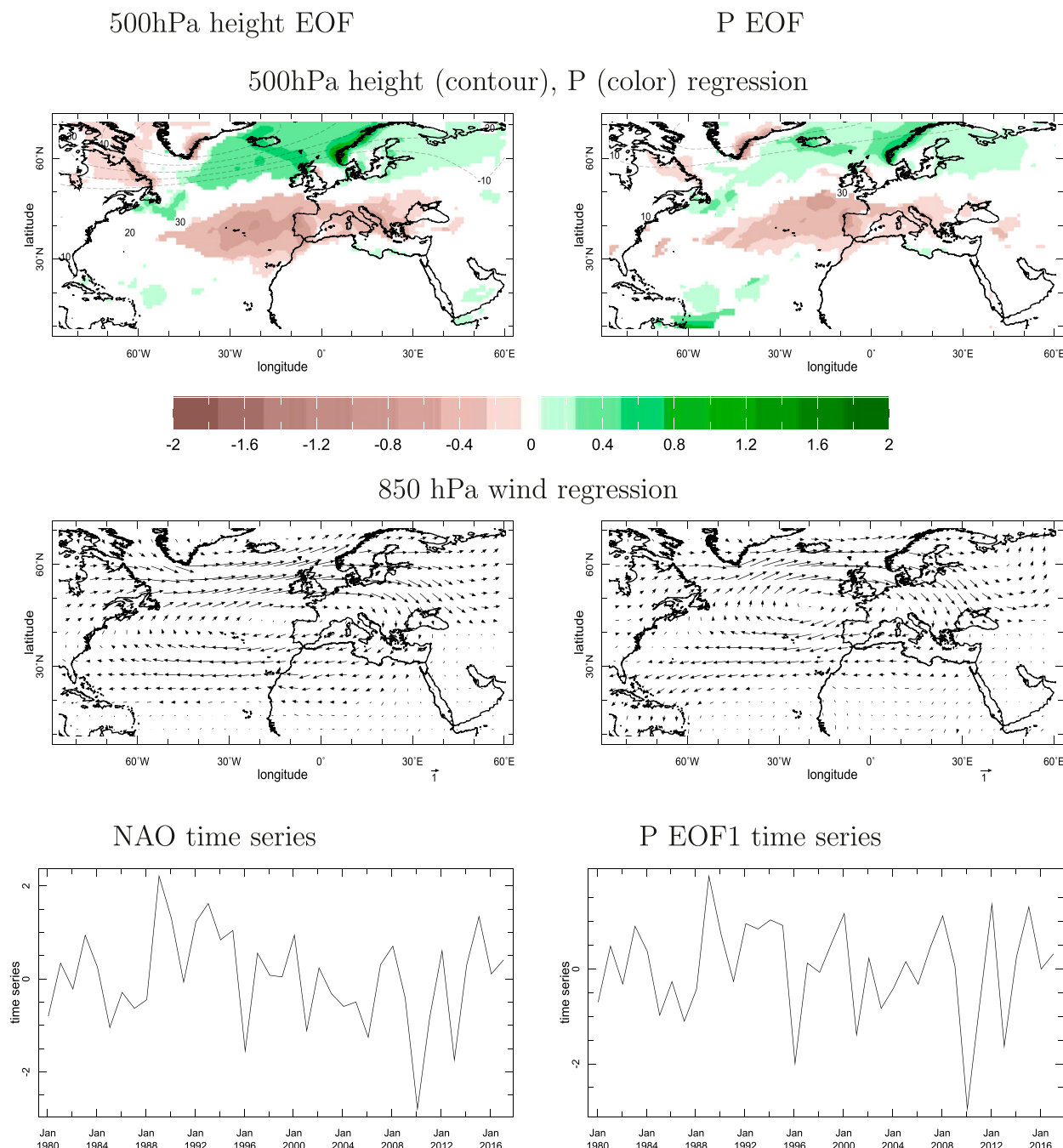
FIG. 1. Patterns of winter (DJFM) 500-hPa height (contours) and precipitation (colors) obtained for (top left) an EOF analysis of 500-hPa heights and (top right) an EOF analysis of precipitation, and (bottom) regression on the associated time series based on ERA-Interim data (the marked year refers to the January of the winter mean). Also shown is the (middle) regressions of the 850-hPa wind vectors. Units are hectopascals, meters per second, and millimeters per month per standard deviation of the time series. The correlation coefficient between the time series is 0.94.
