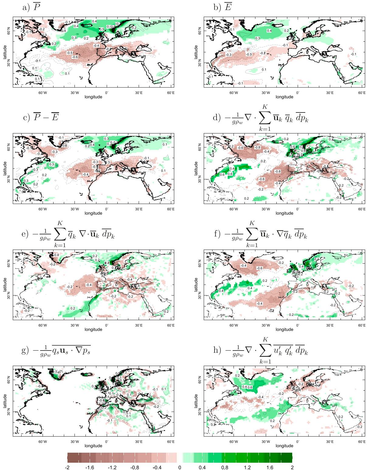
FIG. 4. Terms in the moisture budget regressed onto the NAO index for (a) P , (b) E , (c) P - E , (d) convergence of vertically integrated mean flow moisture flux, and the components related to (e) mass convergence, (f) moisture advection, and (g) the surface term, along with (h) the convergence of vertically integrated eddy moisture flux. Color shading is added where the anomalies are significant at the 95% level according to a two-tailed t test. Time period is winter (DJFM) 1979–2017. All units are millimeters per day.
