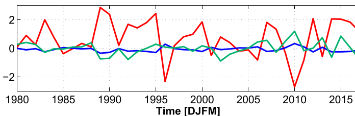
FIG. 6. The observed satellite–gauge precipitation anomaly over land (color shading; \text{mm day}^{-1} ) and 500-hPa height (contours; m) for the most extreme (top left) positive and (top right) negative winters since 1979. Also shown are (bottom) the NAO index, the observed precipitation, and that accounted for by the NAO for Glasgow, Bergen, Madrid, and Belgrade as labeled, together with the respective correlation coefficients between the NAO and observed precipitation. The NAO is in standardized units, and the precipitation in millimeters per day.
