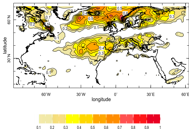
FIG. 2. The fraction of variance in winter (DJFM) precipitation over 1979–2017 explained by the NAO based on ERA-Interim data.
