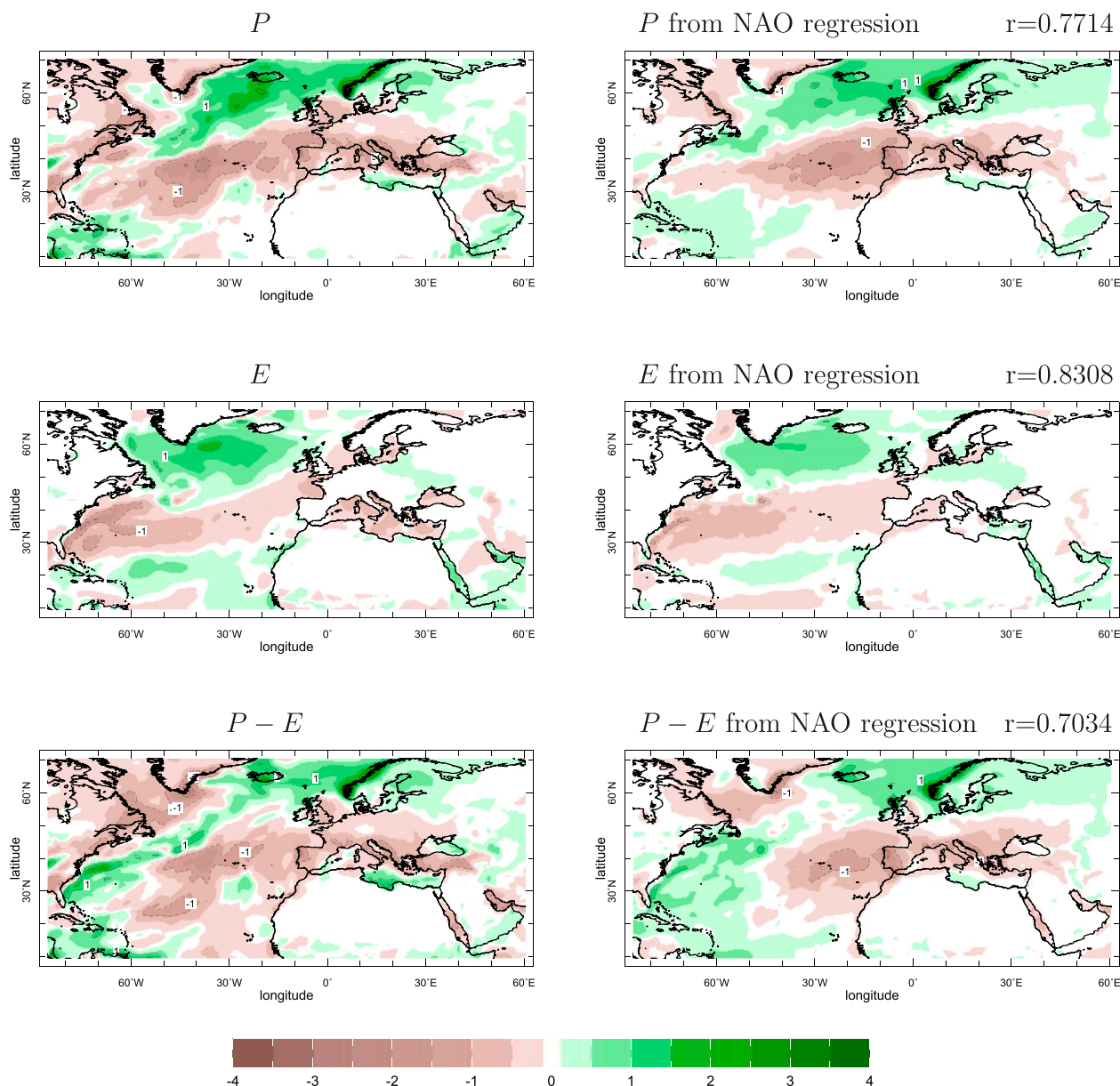
FIG. 7. (left) The reanalysis (top) P , (middle) E , and (bottom) P - E anomalies for the extreme positive NAO winter (DJFM) of 1988/89 and (right) the corresponding component attributable to the NAO anomaly. Area-weighted spatial pattern correlation coefficients between observed and NAO-attributed patterns are shown above the right panels. All units are millimeters per day.
