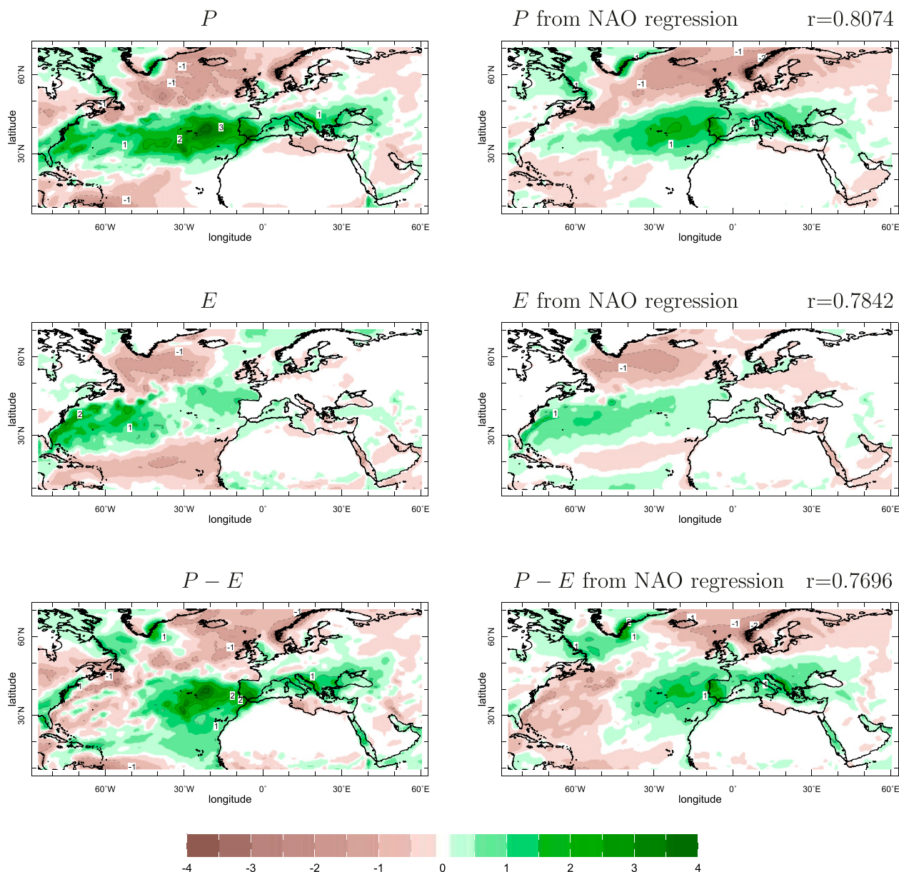
FIG. 9. As in Fig. 7, but for the extreme negative NAO winter (DJFM) of 2009/10.
