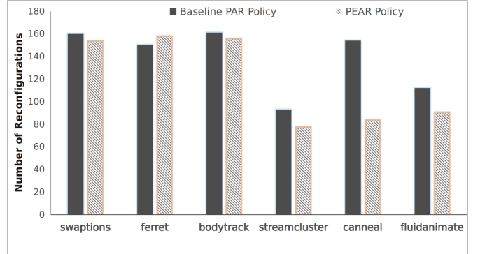
Fig. 3: Comparison of number of HMP reconfigurations required by PAR and PEAR policies.
