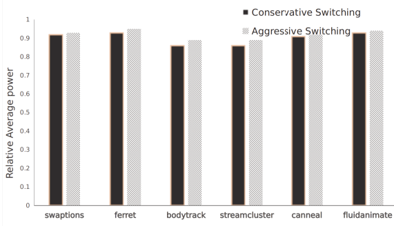
(a) NLANR job arrival: Tight QoS
