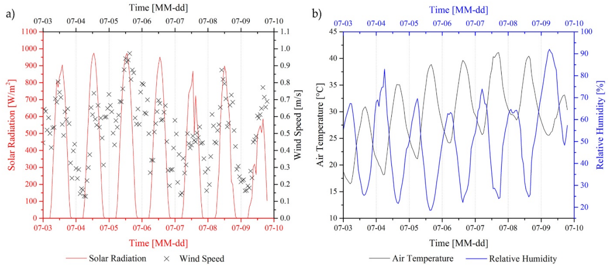
Figure 1. Simulation weather forcing in terms of: (a) incoming global radiation and wind speed; and (b) observed air temperature and relative humidity.
