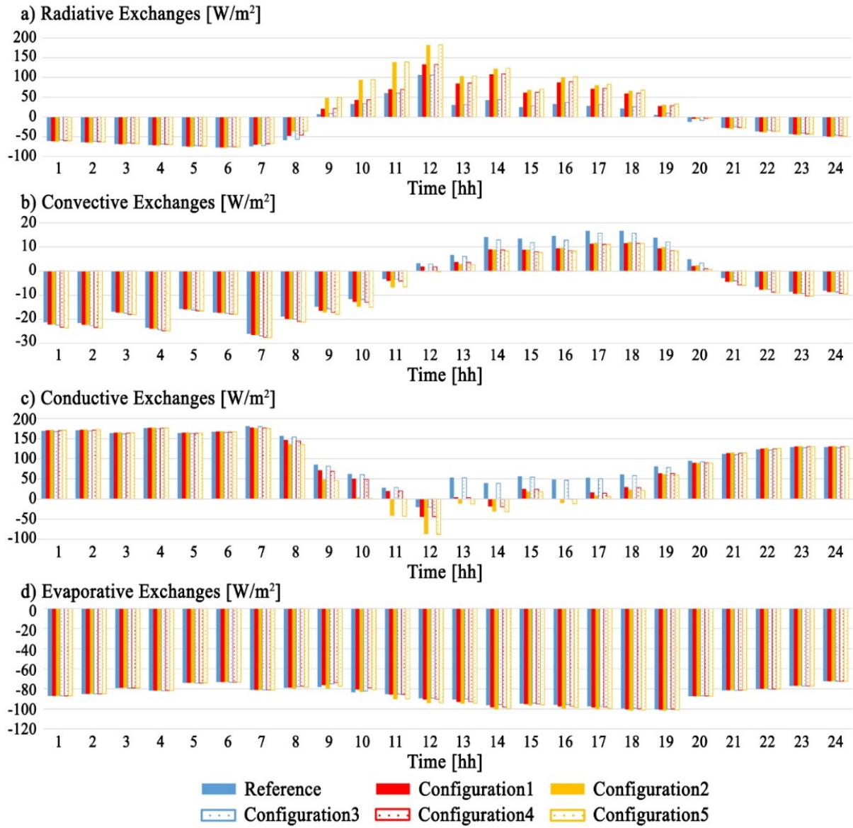
Figure 6. Hourly contribution for all the six simulated configurations of each component of the human energy balance: (a) radiation, (b) convection, (c) conduction, and (d) evaporation.
