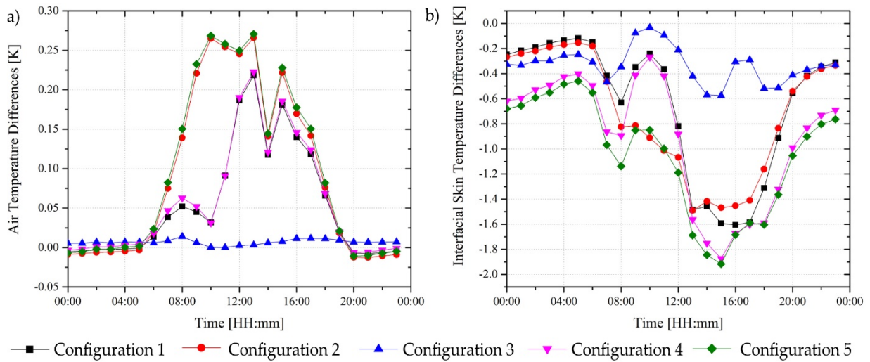
Figure 5. Hourly differentials from the mitigated configurations with respect to reference scenario for the hottest simulated day of: (a) air temperature and (b) interfacial skin temperature.
