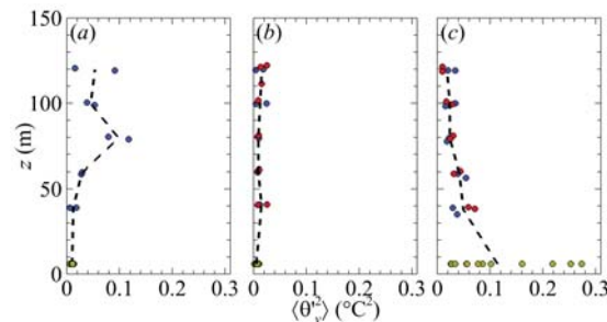
Figure 8. Vertical profiles of potential temperature variance measured during (a) flight 1, (b) flight 2, and (c) flight 3. The blue symbols indicate measurements made by BC5A, the red symbols indicate measurements made by BC5B and the olive symbols indicate measurements made by the sonic anemometer. The dashed line indicates the trend produced by averaging measurements at each altitude.
