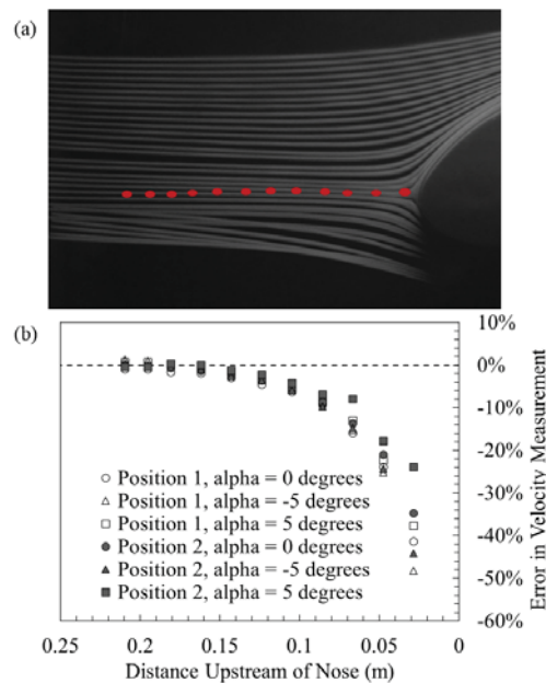
Figure 3. Results of investigation of airframe influence on flow field: (a) scale-model flow visualization, and (b) full-scale wind tunnel comparison of measured velocity to true velocity. Red dots in (a) correspond to streamwise measurement locations in (b).
