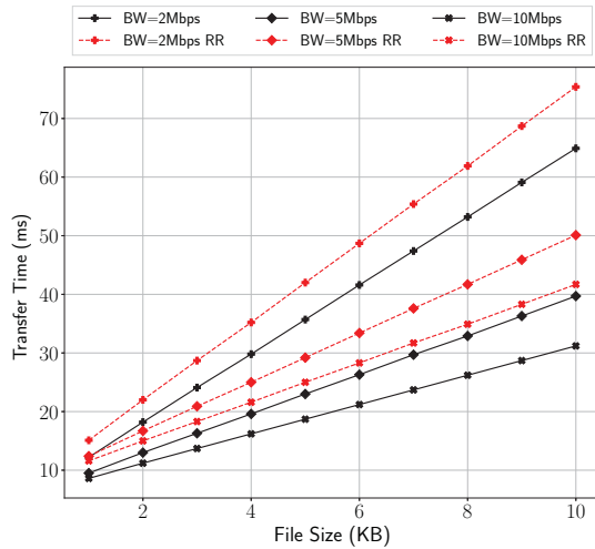
Fig. 4. Transfer time for NDN with and without the router redirection (RR) approach and for different file sizes and client bandwidths
