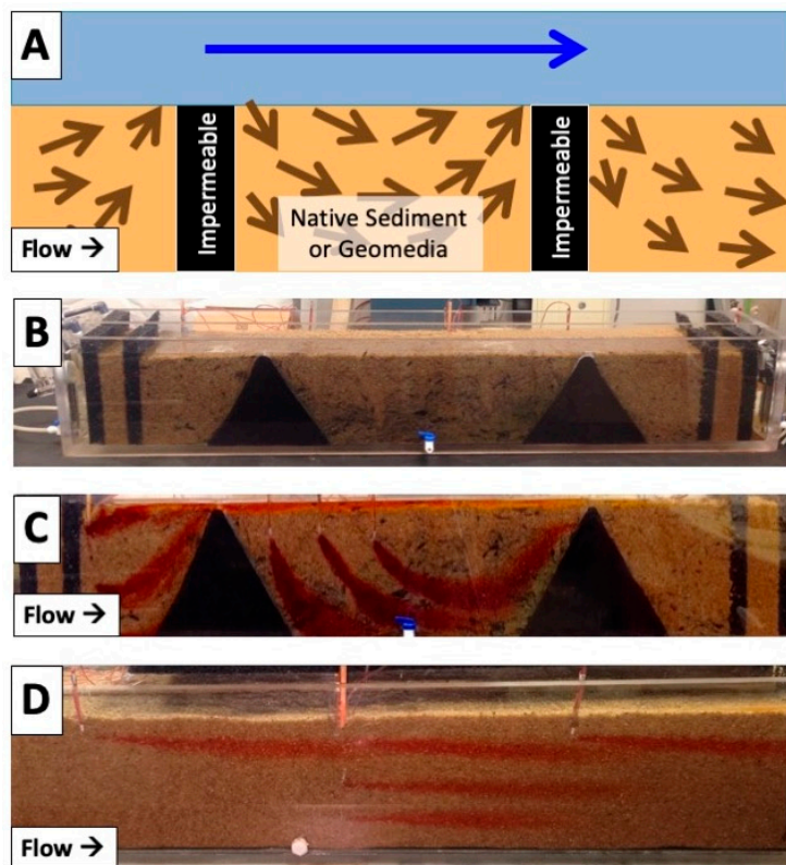
Figure 1. (A) Conceptual diagram of flow in and out of the BEST module, (B) BEST tank with two impermeable triangles installed and sand/woodchip geomedia mix, and (C) red dye showing BEST creating hyporheic exchange compared to (D) control tank with no exchange. Each tank measures 178 cm long, 28 cm deep, and 13 cm wide (text and caption exactly as shown to the interviewees upon request).
