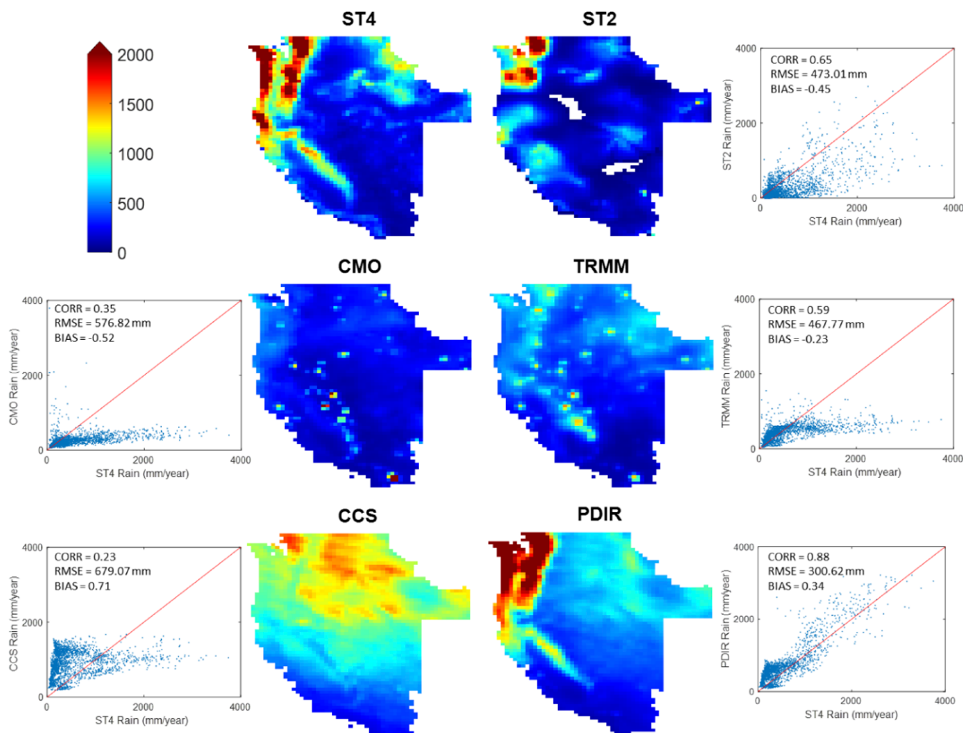
Fig. 4. Average annual rainfall ( \text{mm year}^{-1} ) for the validation period (2008–13) for the baseline product Stage IV (ST4), the near-real-time Stage II (ST2), the three satellite-based precipitation products [CMORPH (CMO), TRMM, and PERSIANN-CCS (CCS)], and the new product, PDIR.
