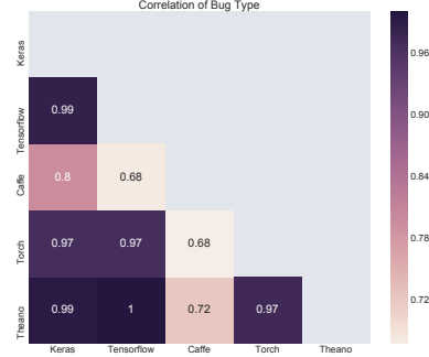
Figure 6: Correlation of Bug Types among the libraries
