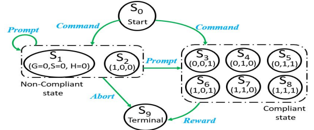
Fig. 5. Naive MDP model: 0 and 1 indicate the presence and absence of a specific observation, respectively
