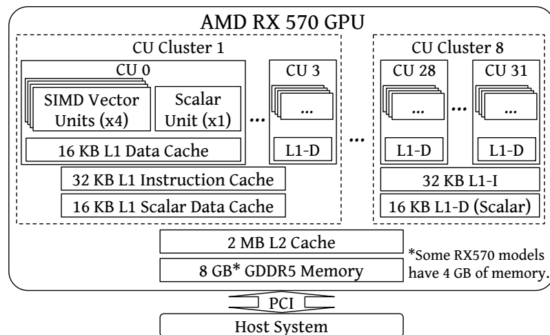
■ Figure 1 Organization of the AMD RX 570 GPU.
