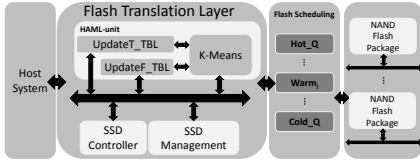
Fig. 5: SSD internal architecture of HAML-SSD design.
