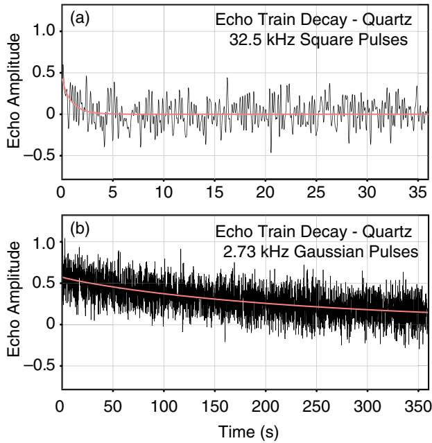
FIG. 3. ^{17}\text{O} CPMG decay of polycrystalline quartz using high-power square and low-power Gaussian pulses. The measured decays are depicted in black while the best-fit stretched exponential decays are depicted in red. The echo train acquisition employed a train of 60 000 \pi pulses with a 6 ms spacing. An rf field strength of \omega_1/(2\pi) = 32.5 kHz was used for the square \pi pulse train while \omega_1/(2\pi) = 2.73 kHz was used for the Gaussian \pi pulse train. Both decays (24 scan average) were filtered in the inverse (frequency) domain with a top-hat filter using cutoffs of \pm 5 Hz. The best fit to exponential decays give T_2 = 1.02 \pm 0.08 s for the higher-power square \pi pulse train decay, and T_2 = 262 \pm 1 s for the lower-power Gaussian \pi pulse train decay. This represents a 260-fold increase in the echo train coherence lifetime. The sensitivity enhancement associated with lowering the rf field strength, determined from the ratio of the initial amplitudes obtained in the fits, is \eta^{\text{lp}} = 1.44 .
