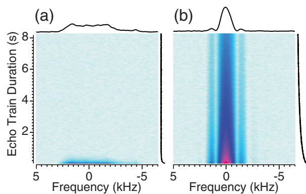
FIG. 1. The ^{17}\text{O} MAS CPMG nuclear spin echo train decay in ^{17}\text{O} -enriched polycrystalline coesite ( \text{SiO}_2 ) at 9.4 T comparing rf field strengths of (a) \omega_1/(2\pi) = 72.5 kHz and (b) 182 Hz. The echo train dimension is on the vertical axis and the frequency dimension is on the horizontal axis. The echo trains follow a stretched exponential decay [11] in (a) with T_2 of 70 \pm 5 ms and a Kohlrausch exponent of \beta = 0.72 \pm 0.03 , and in (b) with T_2 of 2.55 \pm 0.01 s and \beta = 0.542 \pm 0.002 . A T_1 of \sim 400 s was determined and a recovery delay of 600 s was used. In both measurements 1024 \pi pulses were applied with a spacing of \tau_1 = 8 ms and 64 scans were averaged. The one-dimensional (1D) signals above and to the right of each spectrum are the horizontal and vertical cross sections taken at the highest intensity.
