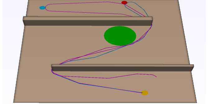
Fig. 8: Planned paths in env.3 for the LTL task specification \varphi_1 in (16) represented by the blue curve and the task specification \varphi_2 in (17) represented by the magenta curve.
