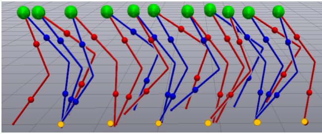
Fig. 9: Walking on level ground using the proposed QP controller. Yellow dots on the ground represent desired stance foot positions.
