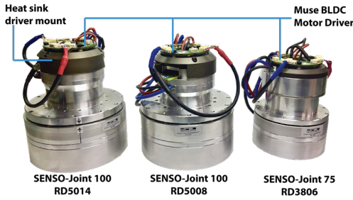
Fig. 8: SENSO-Joint sensor-actuator units from SENSODRIVE assembled with custom BLDC motor controllers by MUSE Robotics used in the ballbot's 7-DoF arm.
