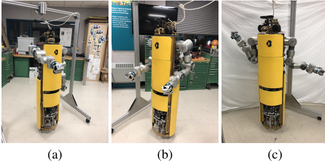
Fig. 15: The enhanced CMU ballbot balancing with the arms in different configurations. Here, a slack rope is attached for safety.
