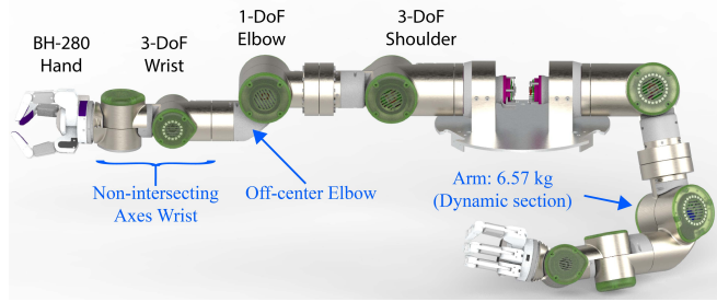
Fig. 2: CMU ballbot dual arm system with BH-282 grippers (CAD rendering).
