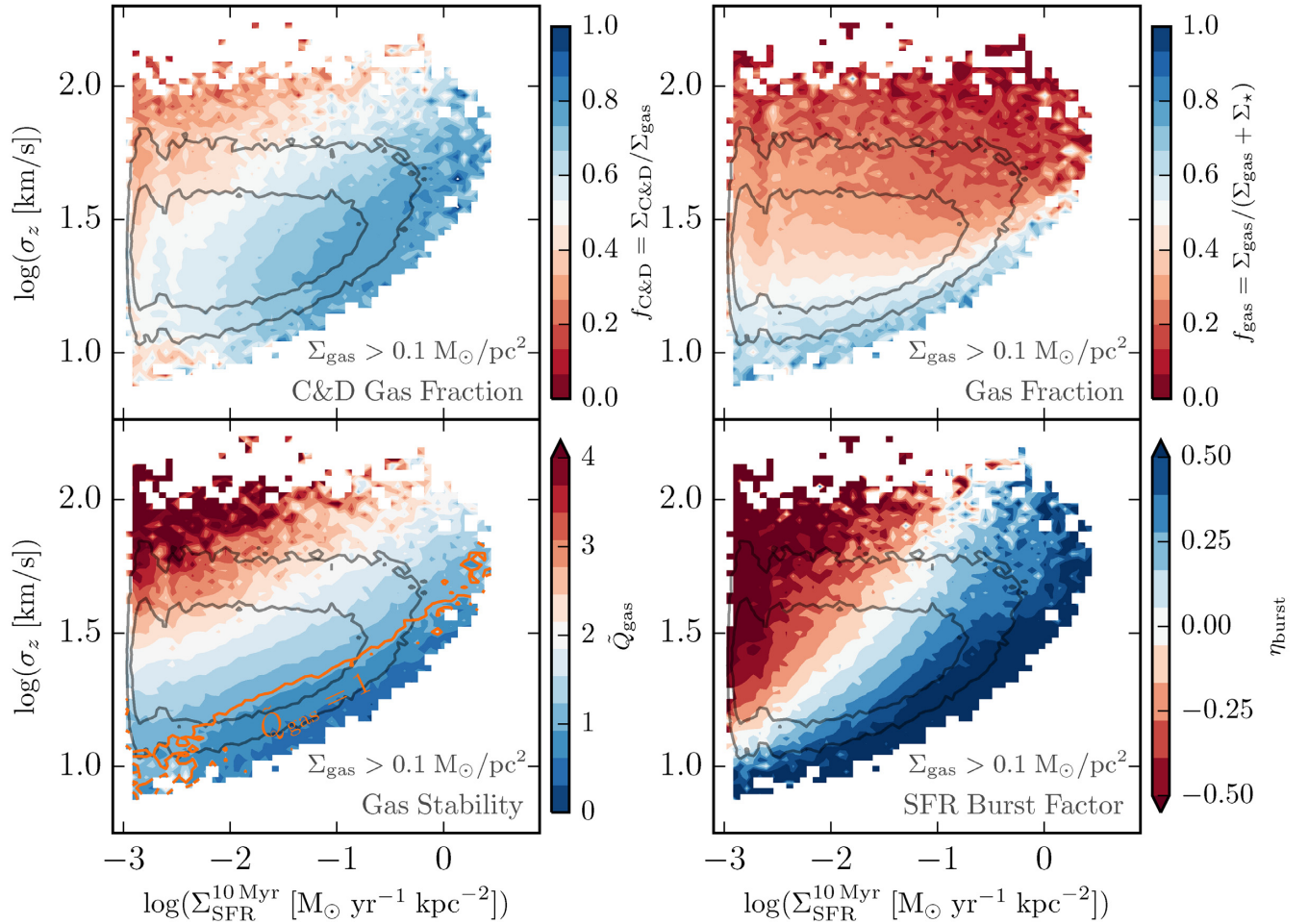
Figure 4. Distribution of \sigma_z and SFR (as Fig. 2, grey contours show 75 and 95 percent data inclusion regions) coloured by various gas and star formation properties on 750 pc scales. Top left: Cold and dense gas fraction ( f_{\text{C\&D}} = \Sigma_{\text{C\&D}} / \Sigma_{\text{gas}} in pixels). C&D gas fraction rises as SFR increases at constant velocity dispersion. Top right: Gas fraction ( f_{\text{gas}} = \Sigma_{\text{gas}} / (\Sigma_{\text{gas}} + \Sigma_{\star}) in pixels). As \Sigma_{\text{SFR}} scales with \Sigma_{\text{gas}} , at fixed \Sigma_{\text{SFR}} lower f_{\text{gas}} is driven by higher \Sigma_{\star} and \Sigma_{\text{tot}} . Gas-rich regions have the lowest velocity dispersions for their SFRs. For a constant amount of gas/star formation, gas in a deeper potential (higher stellar surface densities) must have larger velocity dispersions to maintain stability/equilibrium. Bottom left: Turbulent Toomre- Q parameter \tilde{Q}_{\text{gas}} (equation 1). Orange line denotes \tilde{Q}_{\text{gas}} = 1 threshold for instabilities (i.e. pixels in this region of \Sigma_{\text{SFR}}^{10\text{Myr}} - \sigma_z space are on-average unstable). Less stable gas (at fixed \sigma_z ) produces higher 10 Myr average star formation rates. Bottom right: Star formation ‘burstiness’, \eta_{\text{burst}} . Regions with low ratios of past to current SFRs have low \sigma_z at constant 10-Myr-averaged SFR, corresponding with regions of \tilde{Q}_{\text{gas}} \lesssim 1 .
