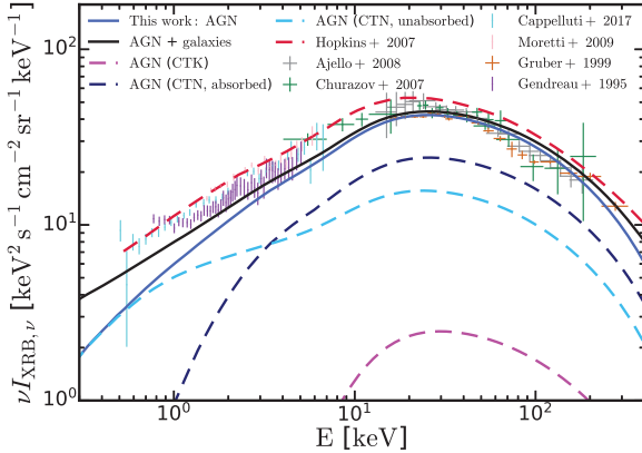
Figure 11. Predicted CXB spectrum. The prediction from our global best-fitting model, which only includes the contribution from quasars, is shown with the blue solid line. The prediction that accounts for a simplified constant 2 \text{ keV}^2 \text{ s}^{-1} \text{ cm}^{-2} \text{ sr}^{-1} \text{ keV}^{-1} contribution from galaxies is shown with the black solid line. The predictions that only include CTN ( \log N_H \geq 24 ) or absorbed CTN ( 22 \leq \log N_H \leq 24 ) or unabsorbed CTN AGN ( \log N_H \leq 22 ) are shown in dashed lines. We compare the predictions to the measurements from Gendreau et al. (1995), Gruber et al. (1999), Churazov et al. (2007), Ajello et al. (2008), Moretti et al. (2009), Cappelluti et al. (2017). We also show the prediction from the Hopkins et al. (2007) model with the red dashed line. The prediction from this work is generally in agreement with the observations despite a \sim 0.05 dex lower at E \lesssim 20 \text{ keV} .
