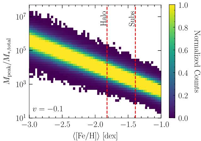
Figure 11. Estimated M_{\text{peak}}/M_{*,\text{total}} - \langle [\text{Fe}/\text{H}] \rangle relation, assuming the growing-scatter model of Garrison-Kimmel et al. (2017a) with v = -0.1 . The average metallicities of the halo and substructure components in the Milky Way, as derived in Necib et al. (2019), are indicated by the red dashed lines.
