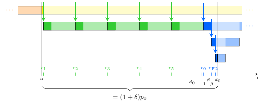
Fig. 2 The structure of the regions and the schedule generated by the region algorithm when faced with the instance \mathcal{I}_m(c) . The darkest shades of a color mean that jobs are scheduled there. The light yellow and blue parts show that the region is currently interrupted. The only time slots where 0 can be processed are the lighter parts of the green regions, i.e., the regions belonging to B(c) (color figure online)
