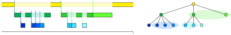
Fig. 1 Gantt chart of the regions (left) and the interruption tree (right) generated by the region algorithm (color figure online)
